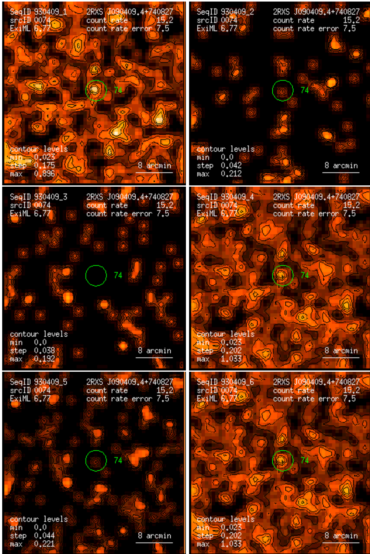
Figure 74: RASS 930409: detection 0074: band rate images, Gaussian filter: (1) PSPC channels 11 – 41, (2) 52 – 90, (3) 91 – 201, (4) 11 – 235, (5) 52 – 201, (6) 11 – 201. Broad band rates in counts/ks. Band rate contour levels in counts/ks/arcmin 2 .
