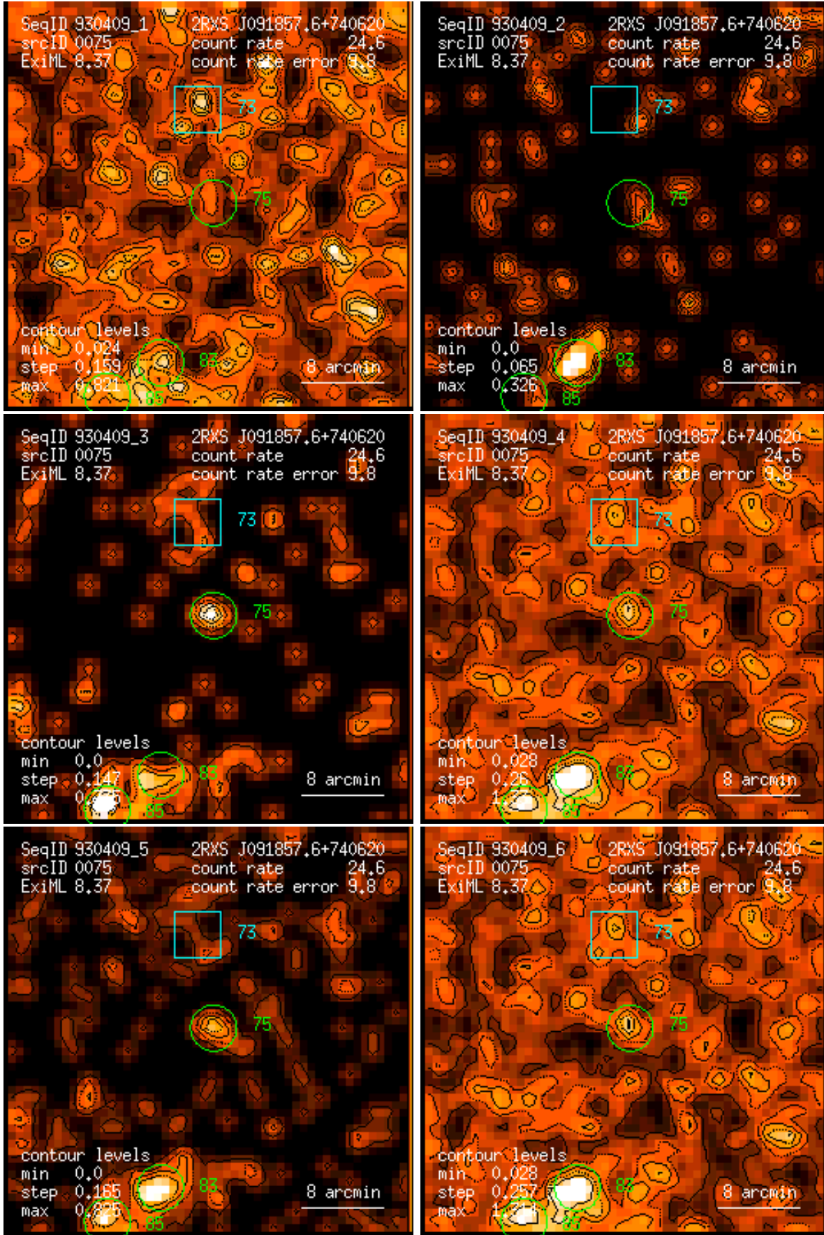
Figure 75: RASS 930409: detection 0075: band rate images, Gaussian filter: (1) PSPC channels 11 – 41, (2) 52 – 90, (3) 91 – 201, (4) 11 – 235, (5) 52 – 201, (6) 11 – 201. Broad band rates in counts/ks. Band rate contour levels in counts/ks/arcmin 2 .
