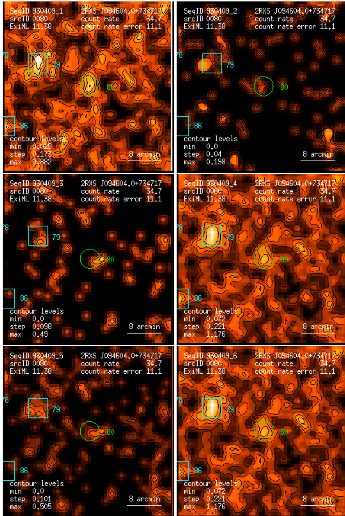
Figure 80: RASS 930409: detection 0080: band rate images, Gaussian filter: (1) PSPC channels 11 – 41, (2) 52 – 90, (3) 91 – 201, (4) 11 – 235, (5) 52 – 201, (6) 11 – 201. Broad band rates in counts/ks. Band rate contour levels in counts/ks/arcmin 2 .
