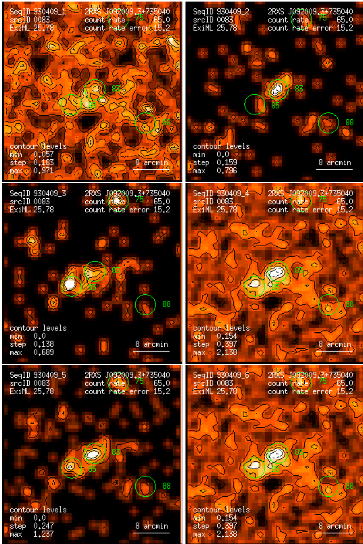
Figure 83: RASS 930409: detection 0083: band rate images, Gaussian filter: (1) PSPC channels 11 – 41, (2) 52 – 90, (3) 91 – 201, (4) 11 – 235, (5) 52 – 201, (6) 11 – 201. Broad band rates in counts/ks. Band rate contour levels in counts/ks/arcmin 2 .
