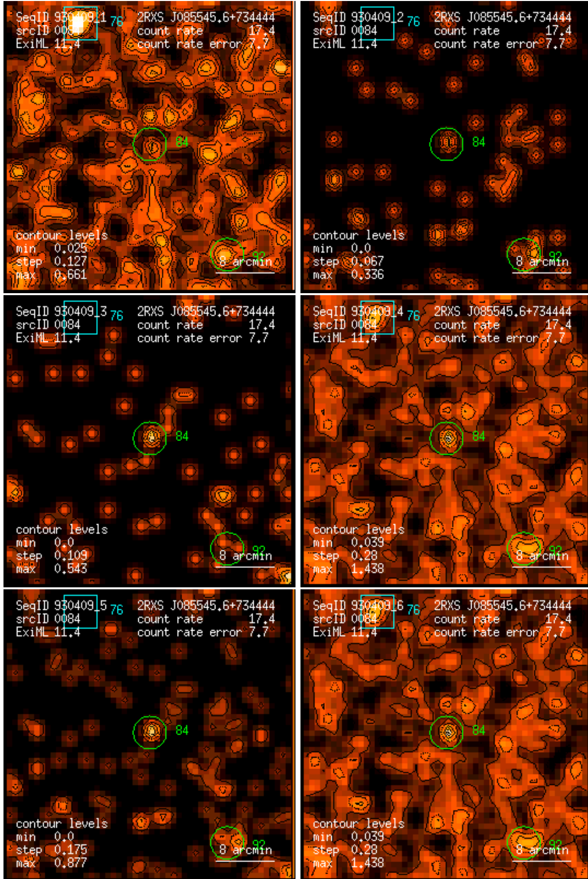
Figure 84: RASS 930409: detection 0084: band rate images, Gaussian filter: (1) PSPC channels 11 – 41, (2) 52 – 90, (3) 91 – 201, (4) 11 – 235, (5) 52 – 201, (6) 11 – 201. Broad band rates in counts/ks. Band rate contour levels in counts/ks/arcmin 2 .
