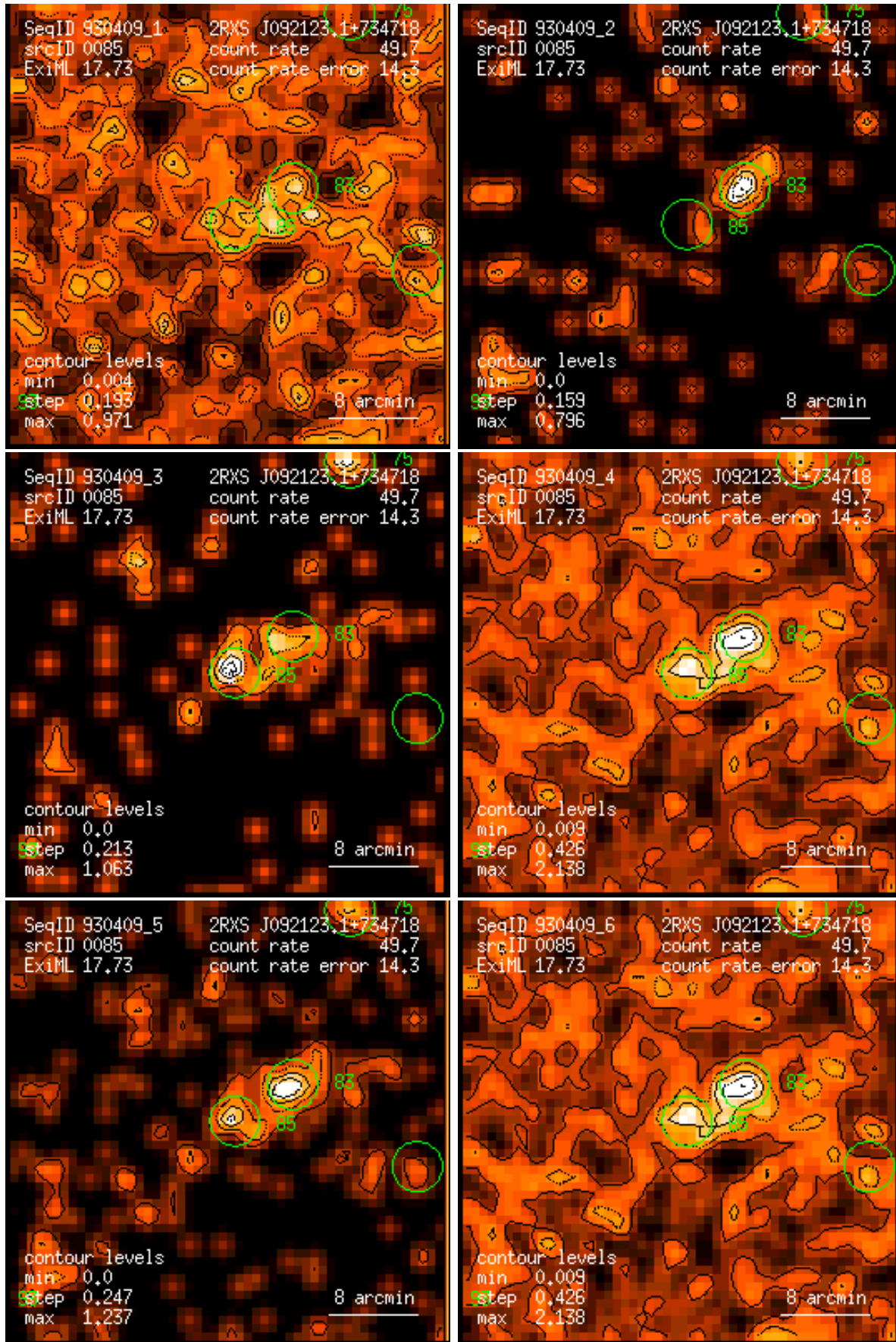
Figure 85: RASS 930409: detection 0085: band rate images, Gaussian filter: (1) PSPC channels 11 – 41, (2) 52 – 90, (3) 91 – 201, (4) 11 – 235, (5) 52 – 201, (6) 11 – 201. Broad band rates in counts/ks. Band rate contour levels in counts/ks/arcmin 2 .
