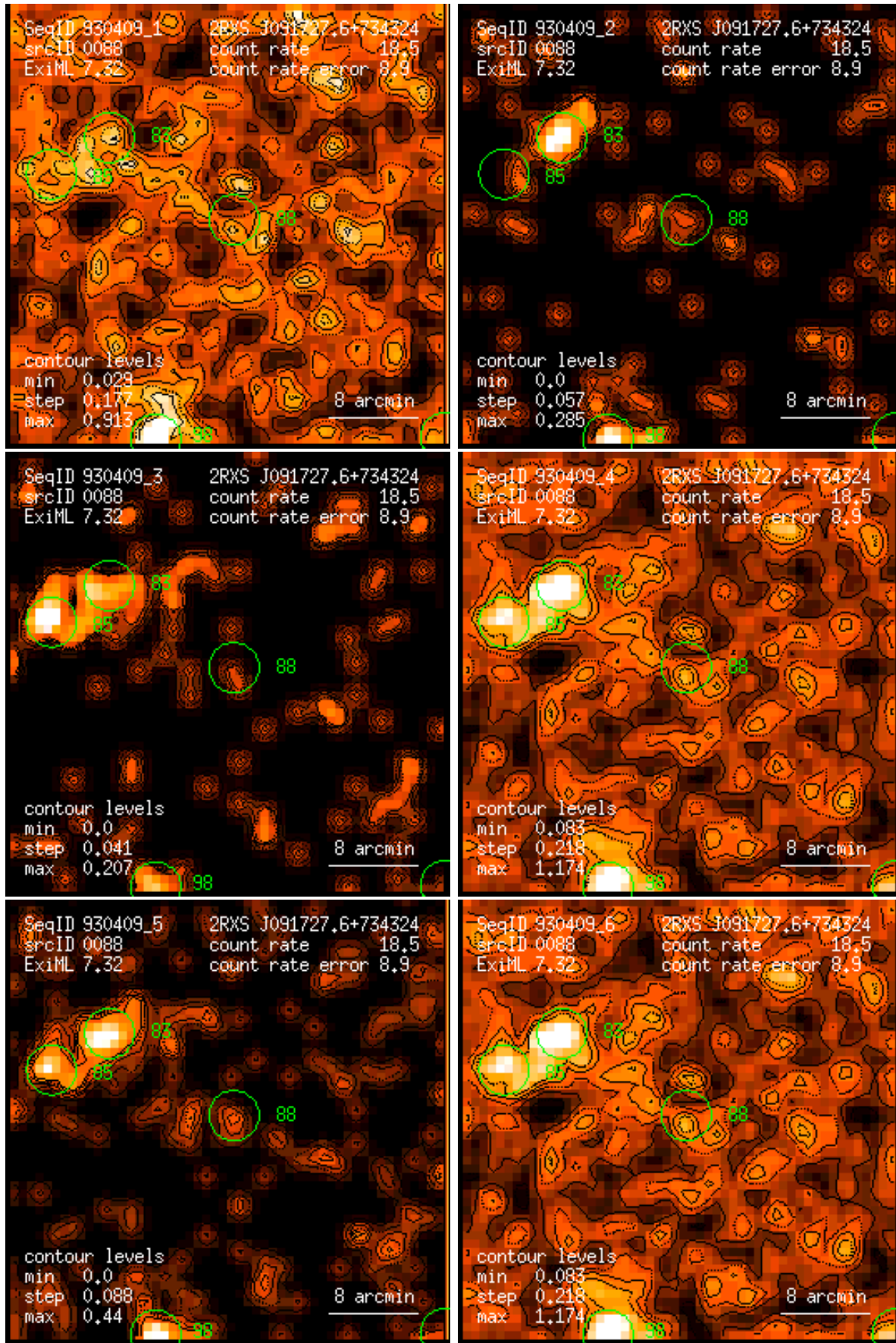
Figure 88: RASS 930409: detection 0088: band rate images, Gaussian filter: (1) PSPC channels 11 – 41, (2) 52 – 90, (3) 91 – 201, (4) 11 – 235, (5) 52 – 201, (6) 11 – 201. Broad band rates in counts/ks. Band rate contour levels in counts/ks/arcmin 2 .
