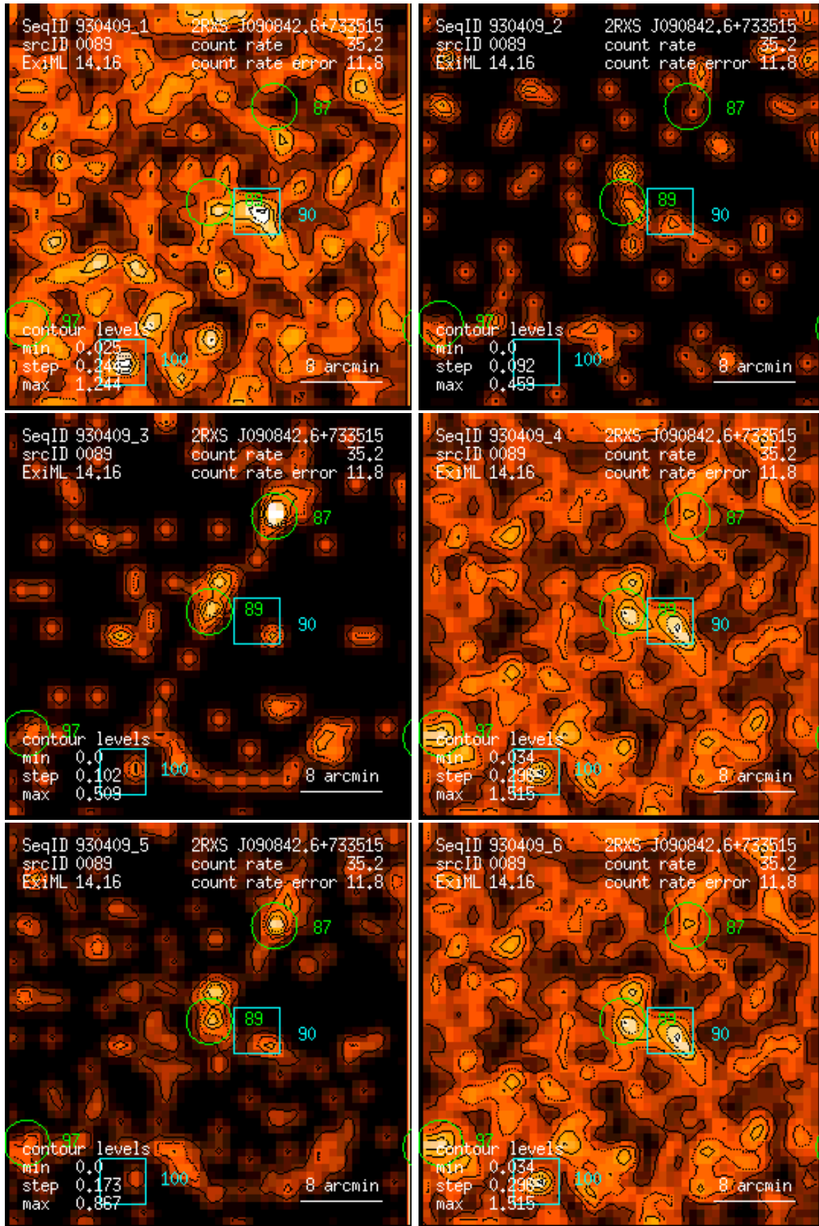
Figure 89: RASS 930409: detection 0089: band rate images, Gaussian filter: (1) PSPC channels 11 – 41, (2) 52 – 90, (3) 91 – 201, (4) 11 – 235, (5) 52 – 201, (6) 11 – 201. Broad band rates in counts/ks. Band rate contour levels in counts/ks/arcmin 2 .
