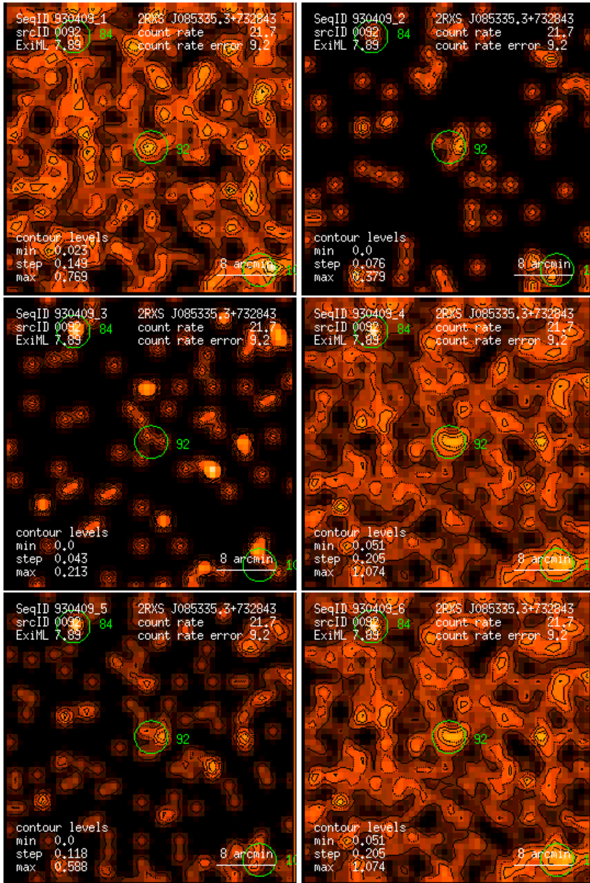
Figure 92: RASS 930409: detection 0092: band rate images, Gaussian filter: (1) PSPC channels 11 – 41, (2) 52 – 90, (3) 91 – 201, (4) 11 – 235, (5) 52 – 201, (6) 11 – 201. Broad band rates in counts/ks. Band rate contour levels in counts/ks/arcmin 2 .
