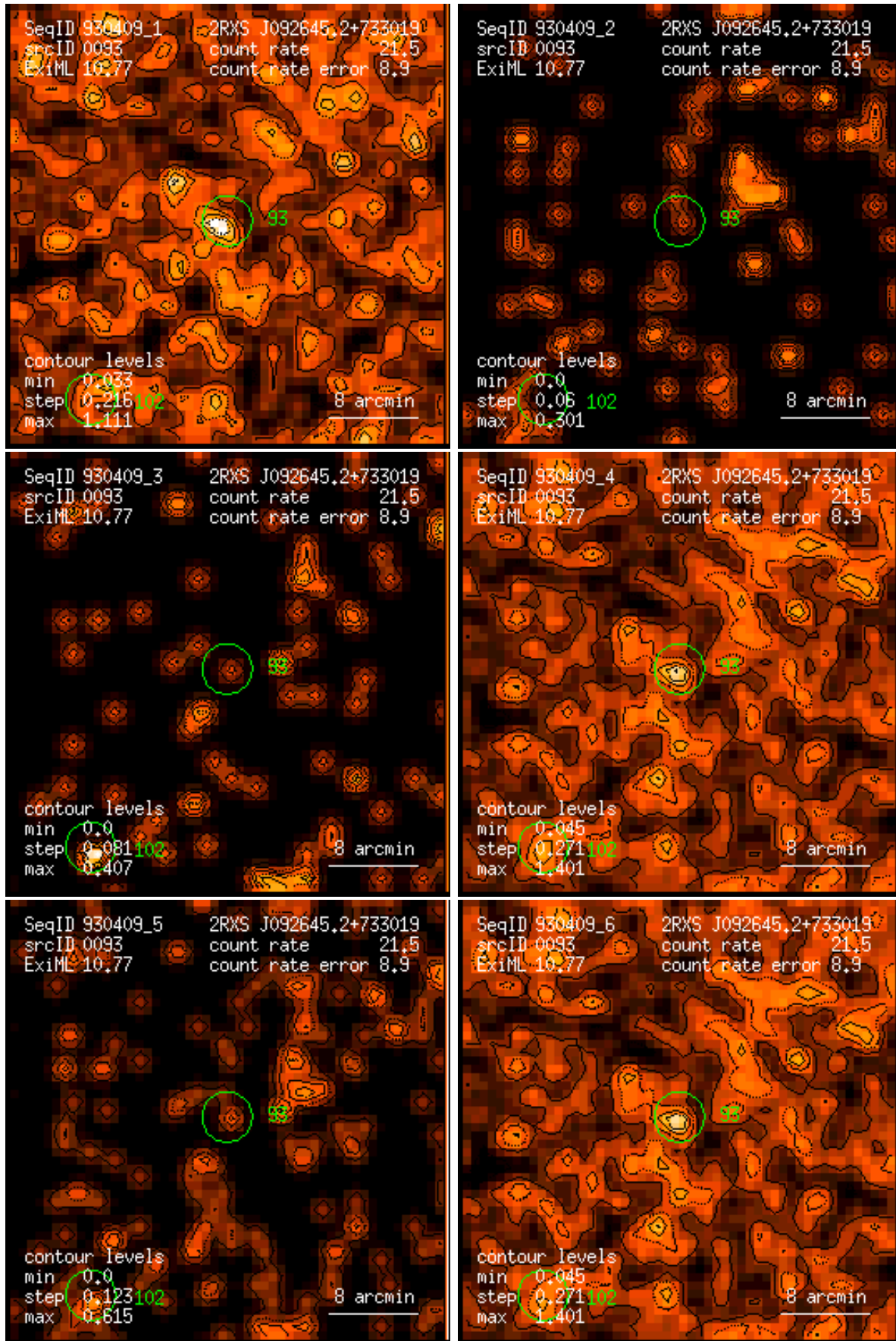
Figure 93: RASS 930409: detection 0093: band rate images, Gaussian filter: (1) PSPC channels 11 – 41, (2) 52 – 90, (3) 91 – 201, (4) 11 – 235, (5) 52 – 201, (6) 11 – 201. Broad band rates in counts/ks. Band rate contour levels in counts/ks/arcmin 2 .
