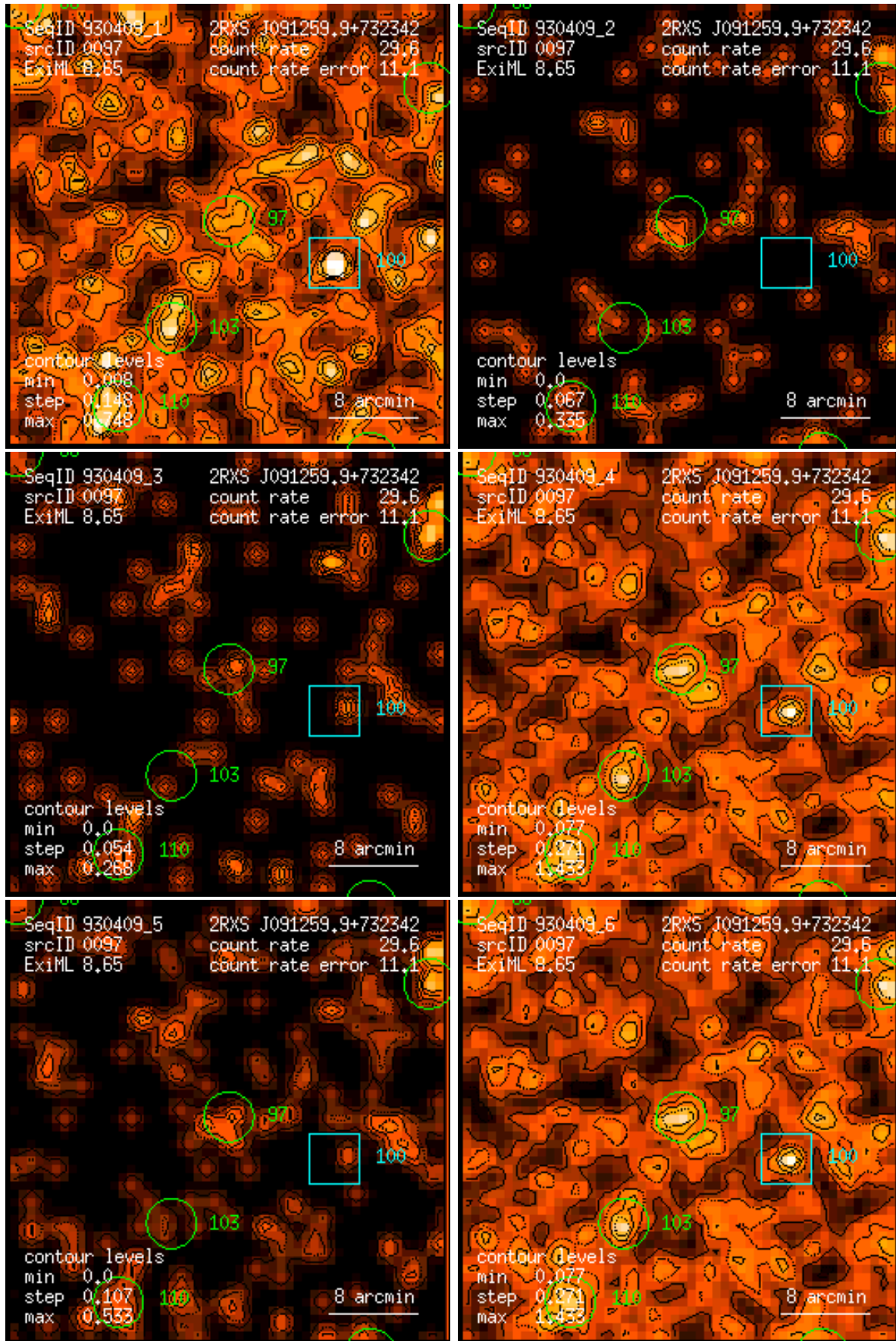
Figure 97: RASS 930409: detection 0097: band rate images, Gaussian filter: (1) PSPC channels 11 – 41, (2) 52 – 90, (3) 91 – 201, (4) 11 – 235, (5) 52 – 201, (6) 11 – 201. Broad band rates in counts/ks. Band rate contour levels in counts/ks/arcmin 2 .
