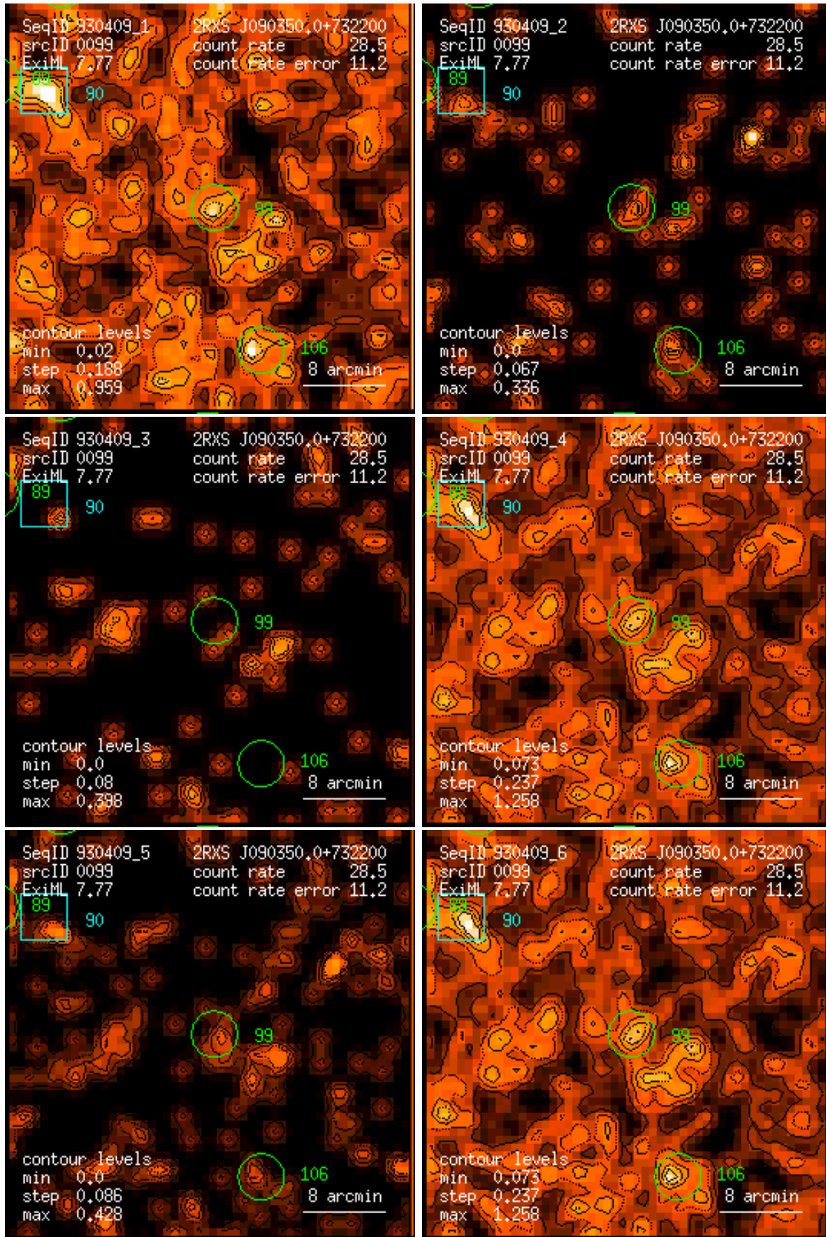
Figure 99: RASS 930409: detection 0099: band rate images, Gaussian filter: (1) PSPC channels 11 – 41, (2) 52 – 90, (3) 91 – 201, (4) 11 – 235, (5) 52 – 201, (6) 11 – 201. Broad band rates in counts/ks. Band rate contour levels in counts/ks/arcmin 2 .
