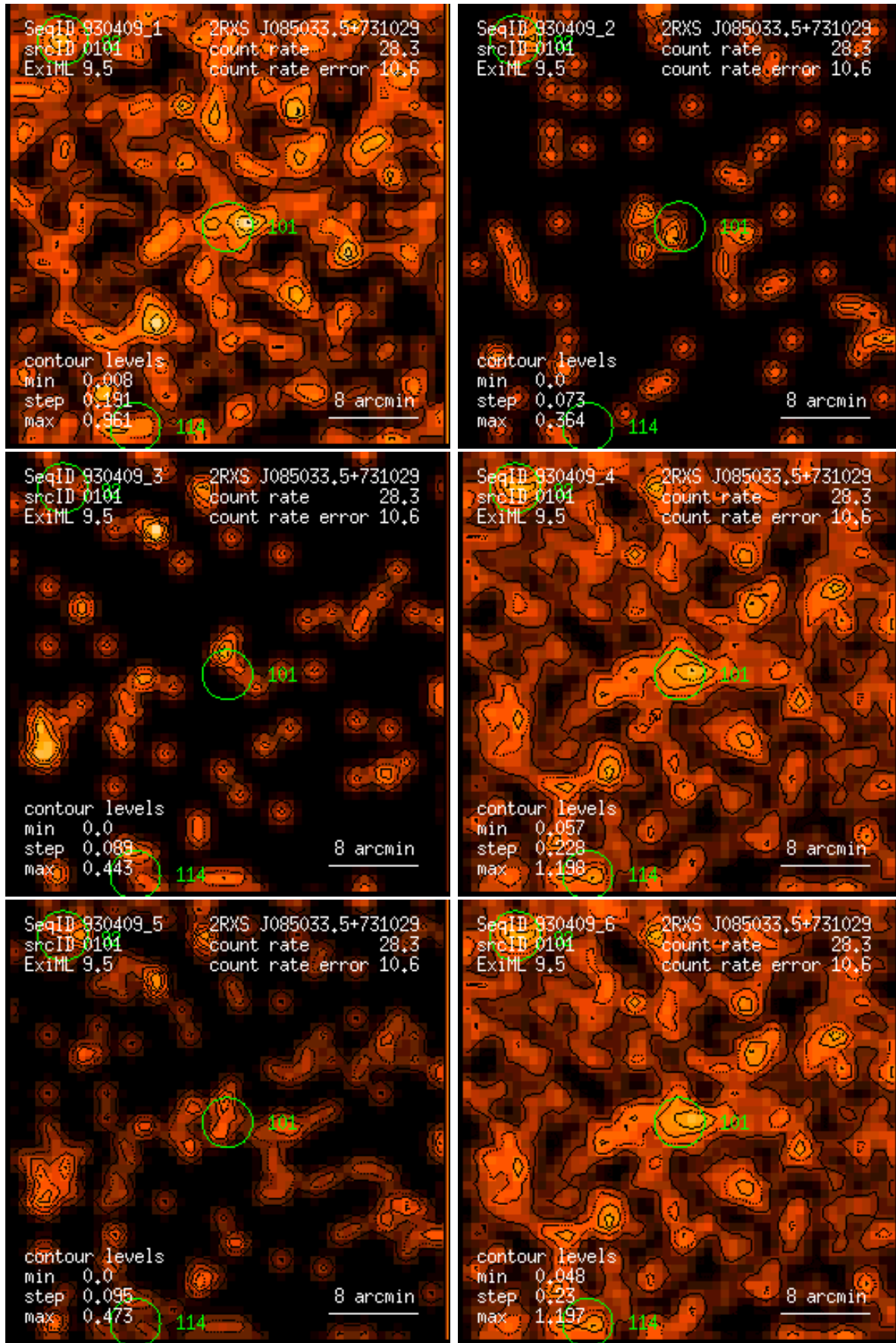
Figure 101: RASS 930409: detection 0101: band rate images, Gaussian filter: (1) PSPC channels 11 – 41, (2) 52 – 90, (3) 91 – 201, (4) 11 – 235, (5) 52 – 201, (6) 11 – 201. Broad band rates in counts/ks. Band rate contour levels in counts/ks/arcmin 2 .
