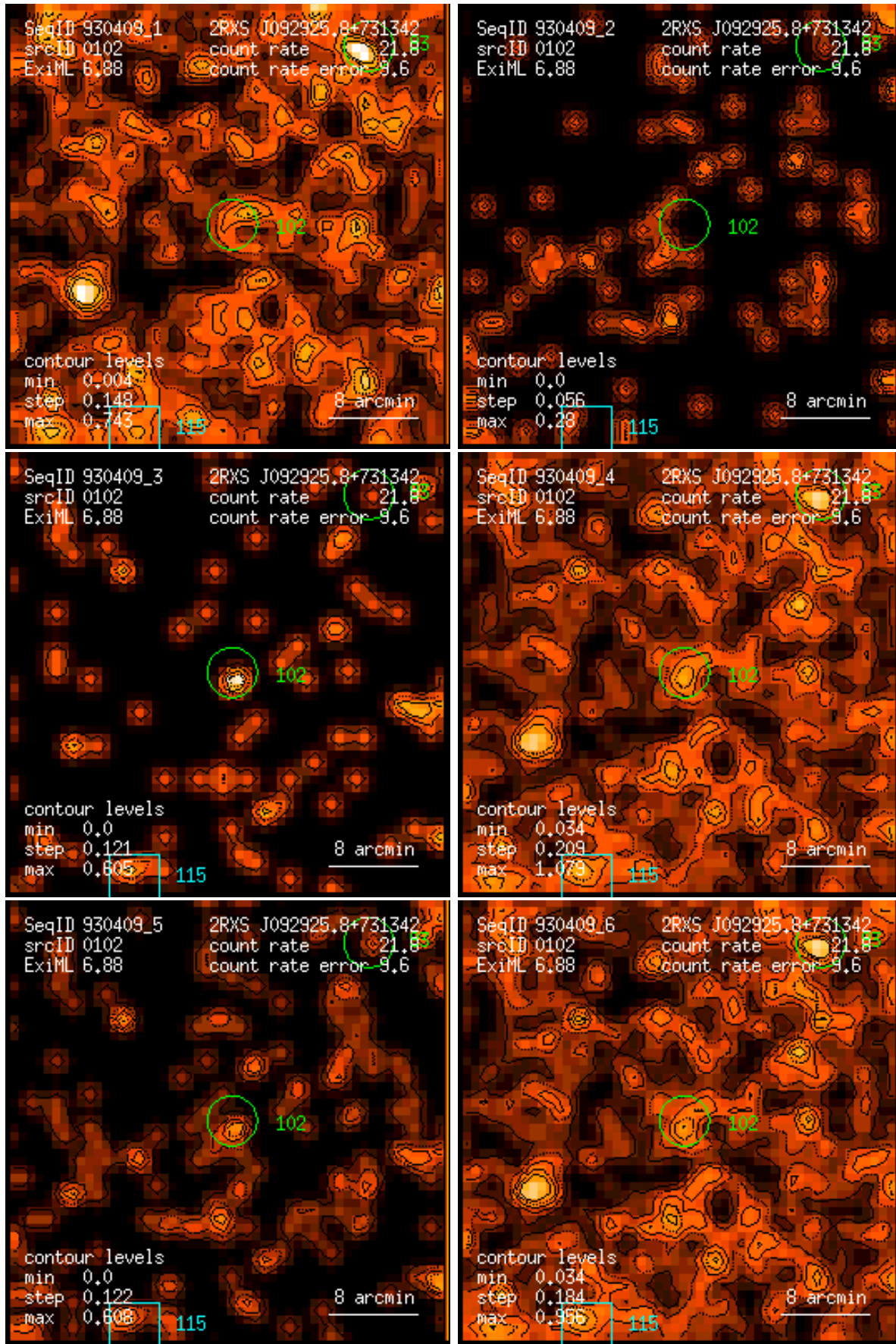
Figure 102: RASS 930409: detection 0102: band rate images, Gaussian filter: (1) PSPC channels 11 – 41, (2) 52 – 90, (3) 91 – 201, (4) 11 – 235, (5) 52 – 201, (6) 11 – 201. Broad band rates in counts/ks. Band rate contour levels in counts/ks/arcmin 2 .
