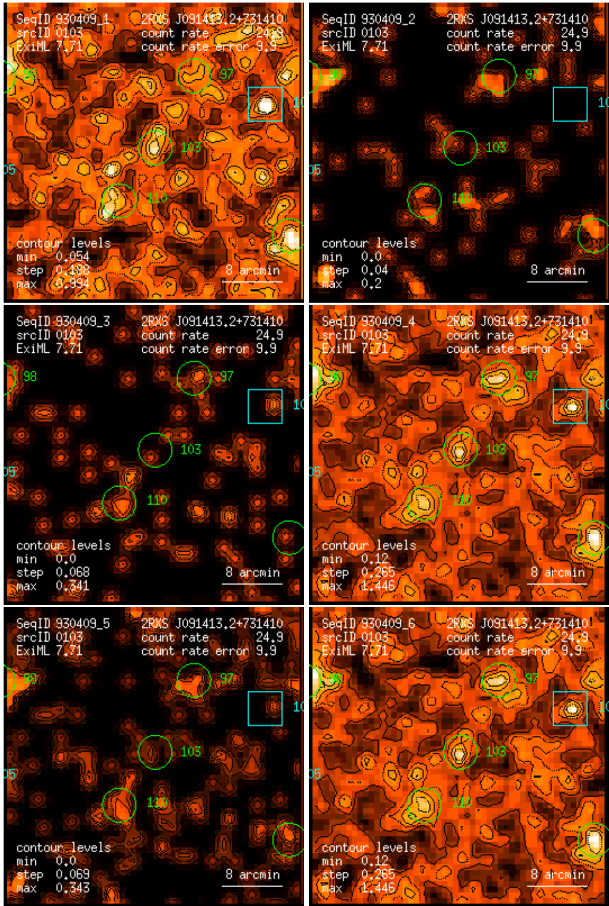
Figure 103: RASS 930409: detection 0103: band rate images, Gaussian filter: (1) PSPC channels 11 – 41, (2) 52 – 90, (3) 91 – 201, (4) 11 – 235, (5) 52 – 201, (6) 11 – 201. Broad band rates in counts/ks. Band rate contour levels in counts/ks/arcmin 2 .
