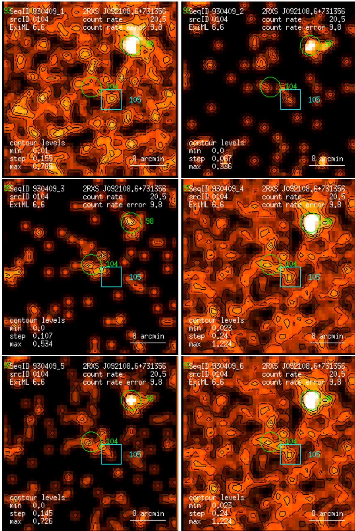
Figure 104: RASS 930409: detection 0104: band rate images, Gaussian filter: (1) PSPC channels 11 – 41, (2) 52 – 90, (3) 91 – 201, (4) 11 – 235, (5) 52 – 201, (6) 11 – 201. Broad band rates in counts/ks. Band rate contour levels in counts/ks/arcmin 2 .
