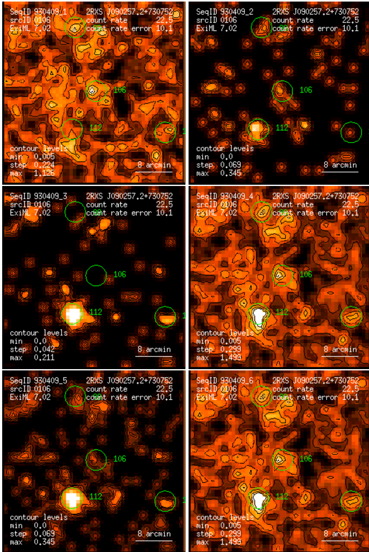
Figure 106: RASS 930409: detection 0106: band rate images, Gaussian filter: (1) PSPC channels 11 – 41, (2) 52 – 90, (3) 91 – 201, (4) 11 – 235, (5) 52 – 201, (6) 11 – 201. Broad band rates in counts/ks. Band rate contour levels in counts/ks/arcmin 2 .
