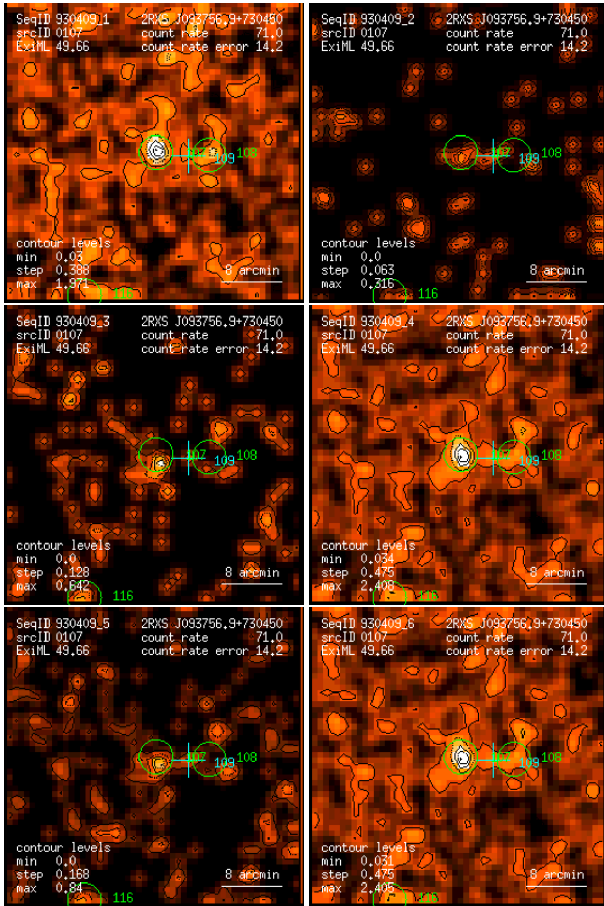
Figure 107: RASS 930409: detection 0107: band rate images, Gaussian filter: (1) PSPC channels 11 – 41, (2) 52 – 90, (3) 91 – 201, (4) 11 – 235, (5) 52 – 201, (6) 11 – 201. Broad band rates in counts/ks. Band rate contour levels in counts/ks/arcmin 2 .
