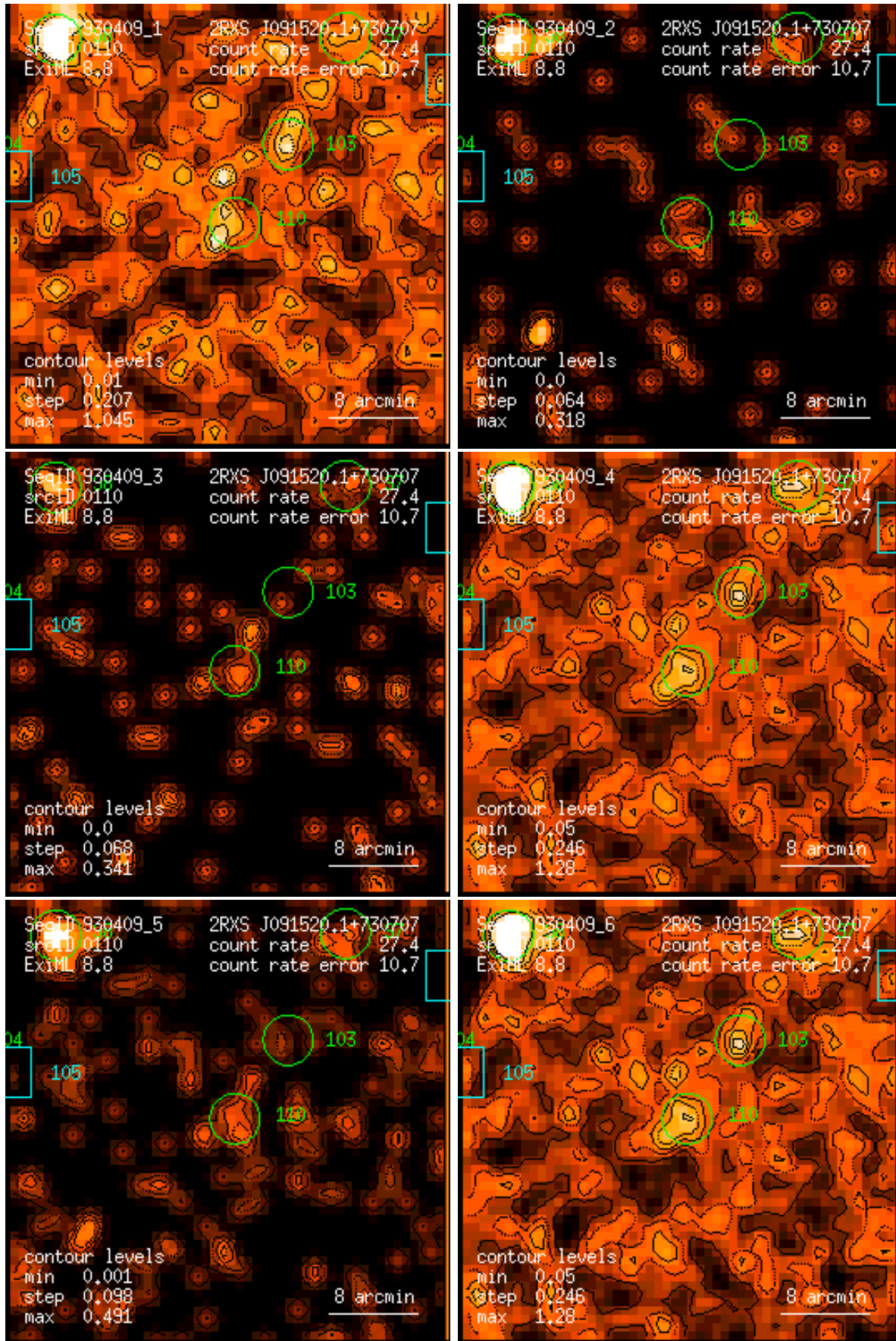
Figure 110: RASS 930409: detection 0110: band rate images, Gaussian filter: (1) PSPC channels 11 – 41, (2) 52 – 90, (3) 91 – 201, (4) 11 – 235, (5) 52 – 201, (6) 11 – 201. Broad band rates in counts/ks. Band rate contour levels in counts/ks/arcmin 2 .
