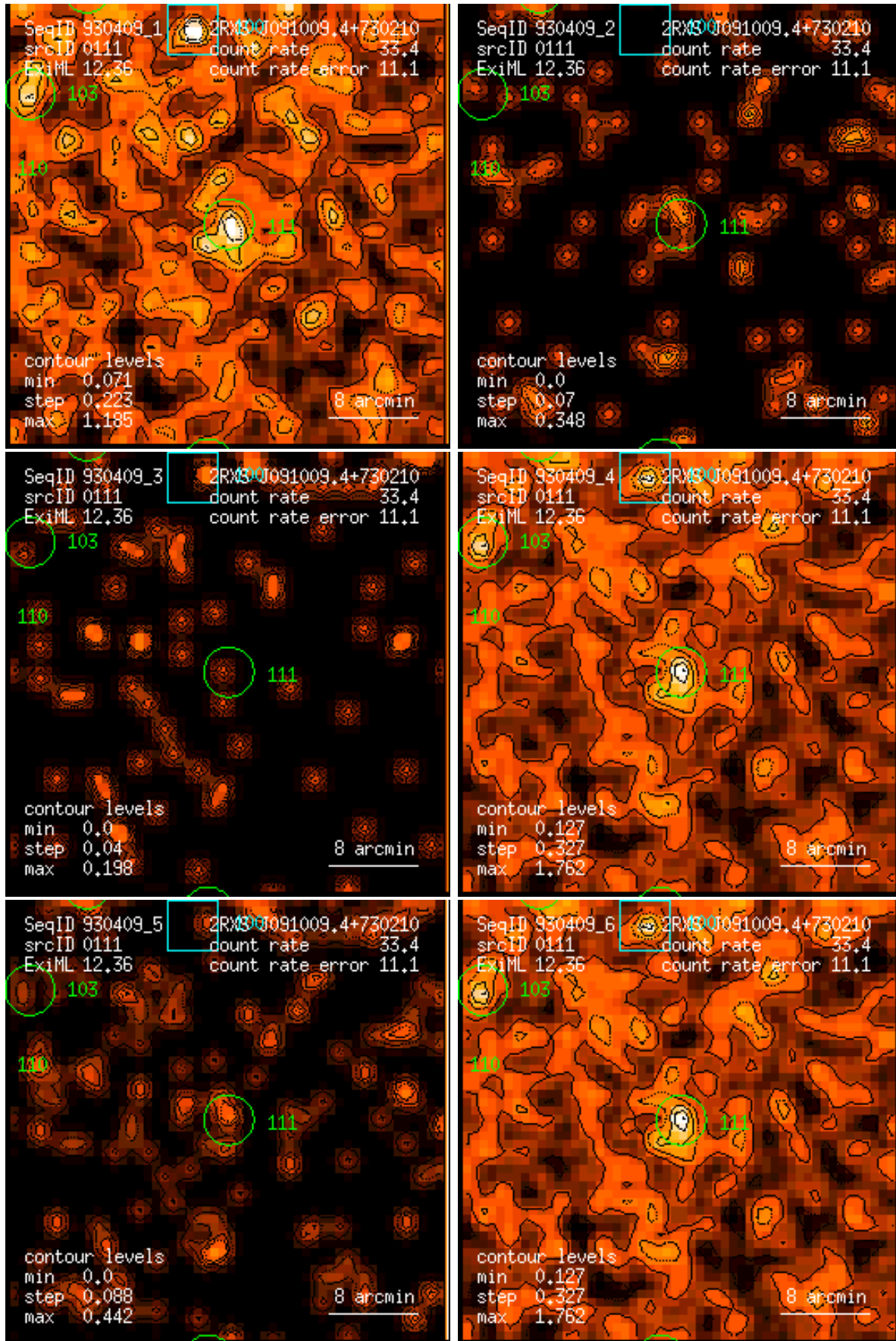
Figure 111: RASS 930409: detection 0111: band rate images, Gaussian filter: (1) PSPC channels 11 – 41, (2) 52 – 90, (3) 91 – 201, (4) 11 – 235, (5) 52 – 201, (6) 11 – 201. Broad band rates in counts/ks. Band rate contour levels in counts/ks/arcmin 2 .
