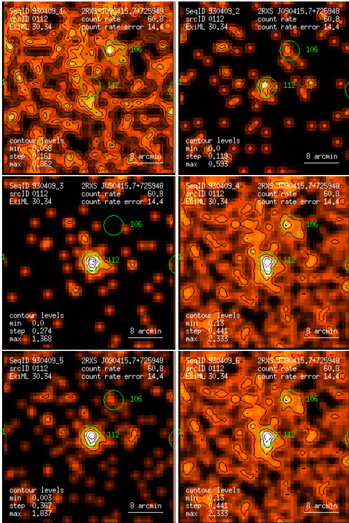
Figure 112: RASS 930409: detection 0112: band rate images, Gaussian filter: (1) PSPC channels 11 – 41, (2) 52 – 90, (3) 91 – 201, (4) 11 – 235, (5) 52 – 201, (6) 11 – 201. Broad band rates in counts/ks. Band rate contour levels in counts/ks/arcmin 2 .
