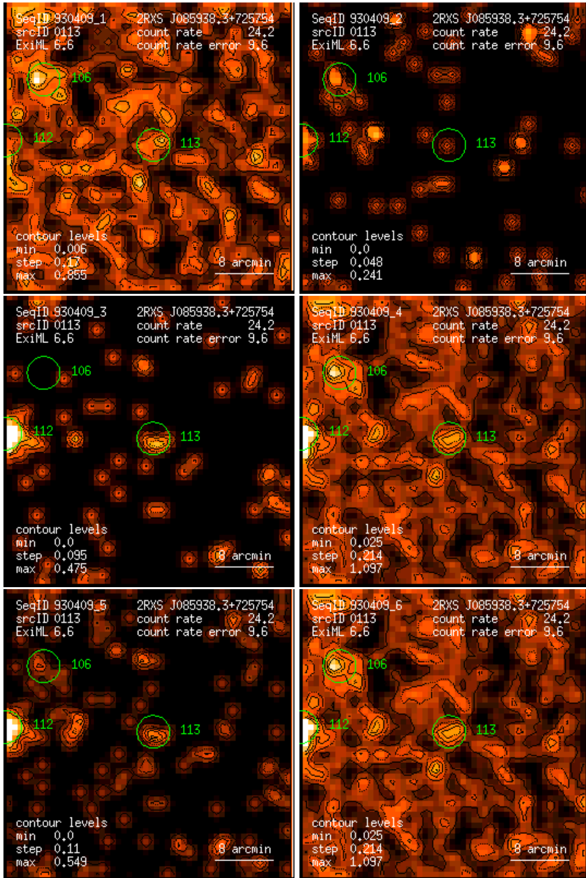
Figure 113: RASS 930409: detection 0113: band rate images, Gaussian filter: (1) PSPC channels 11 – 41, (2) 52 – 90, (3) 91 – 201, (4) 11 – 235, (5) 52 – 201, (6) 11 – 201. Broad band rates in counts/ks. Band rate contour levels in counts/ks/arcmin 2 .
