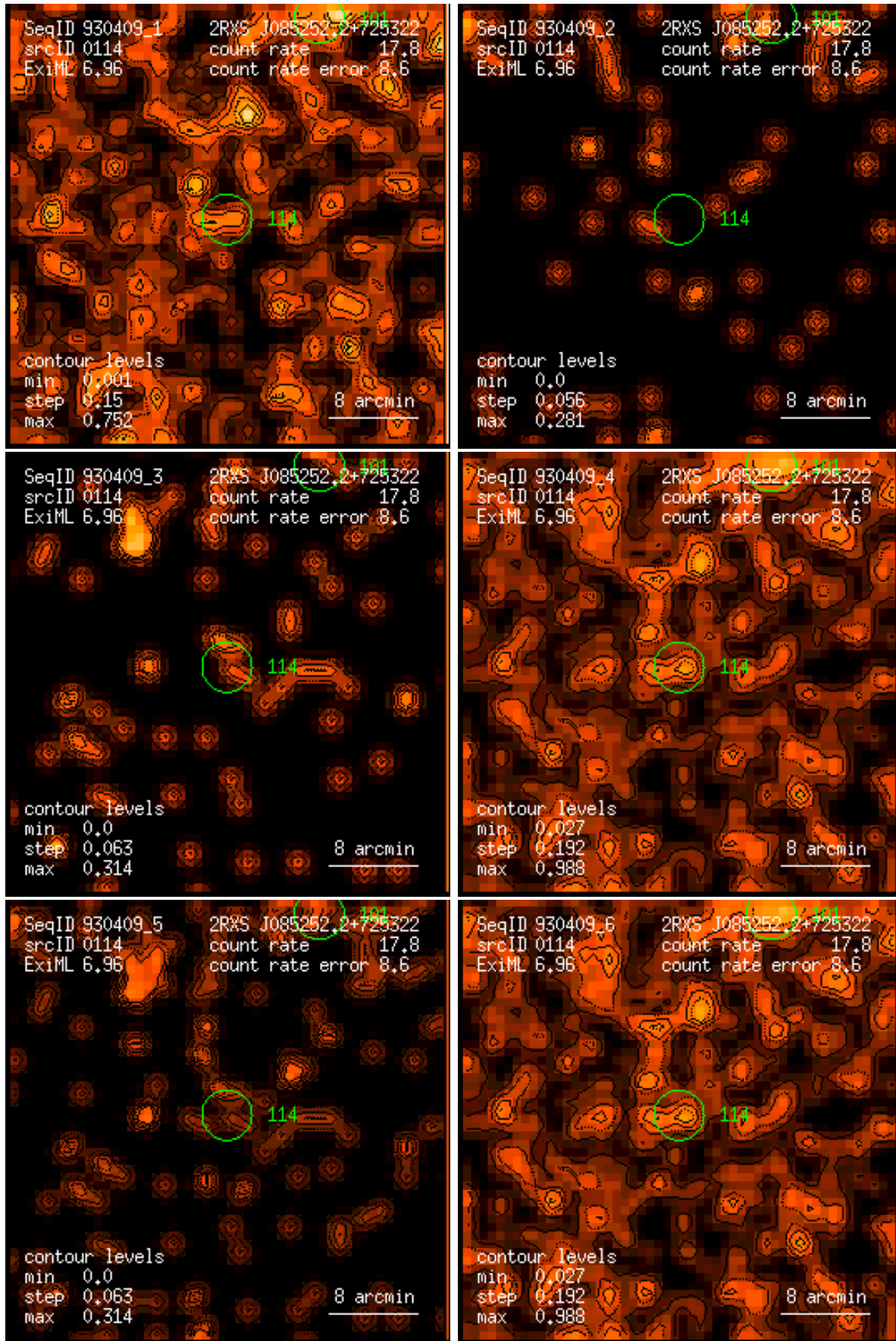
Figure 114: RASS 930409: detection 0114: band rate images, Gaussian filter: (1) PSPC channels 11 – 41, (2) 52 – 90, (3) 91 – 201, (4) 11 – 235, (5) 52 – 201, (6) 11 – 201. Broad band rates in counts/ks. Band rate contour levels in counts/ks/arcmin 2 .
