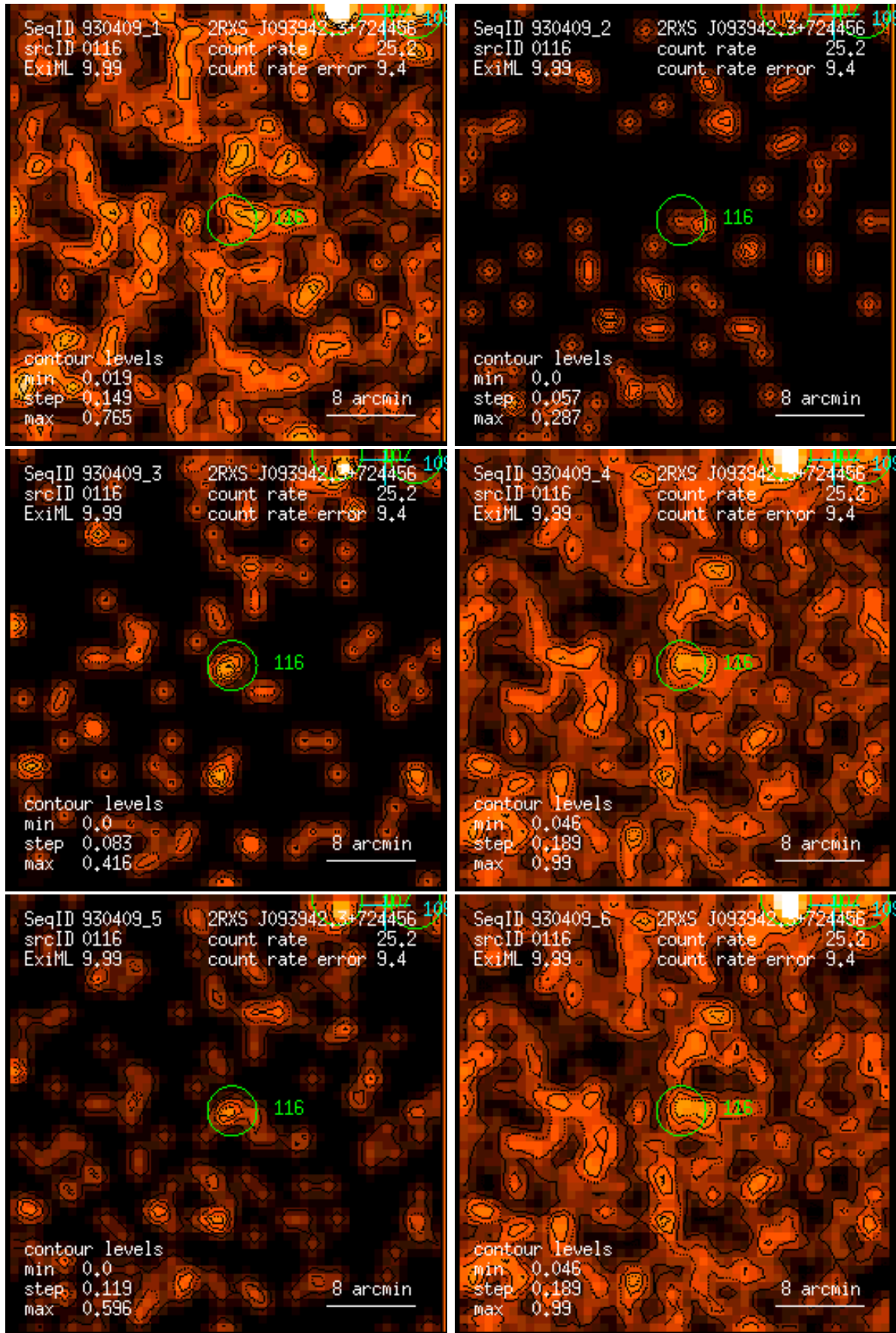
Figure 116: RASS 930409: detection 0116: band rate images, Gaussian filter: (1) PSPC channels 11 – 41, (2) 52 – 90, (3) 91 – 201, (4) 11 – 235, (5) 52 – 201, (6) 11 – 201. Broad band rates in counts/ks. Band rate contour levels in counts/ks/arcmin 2 .
