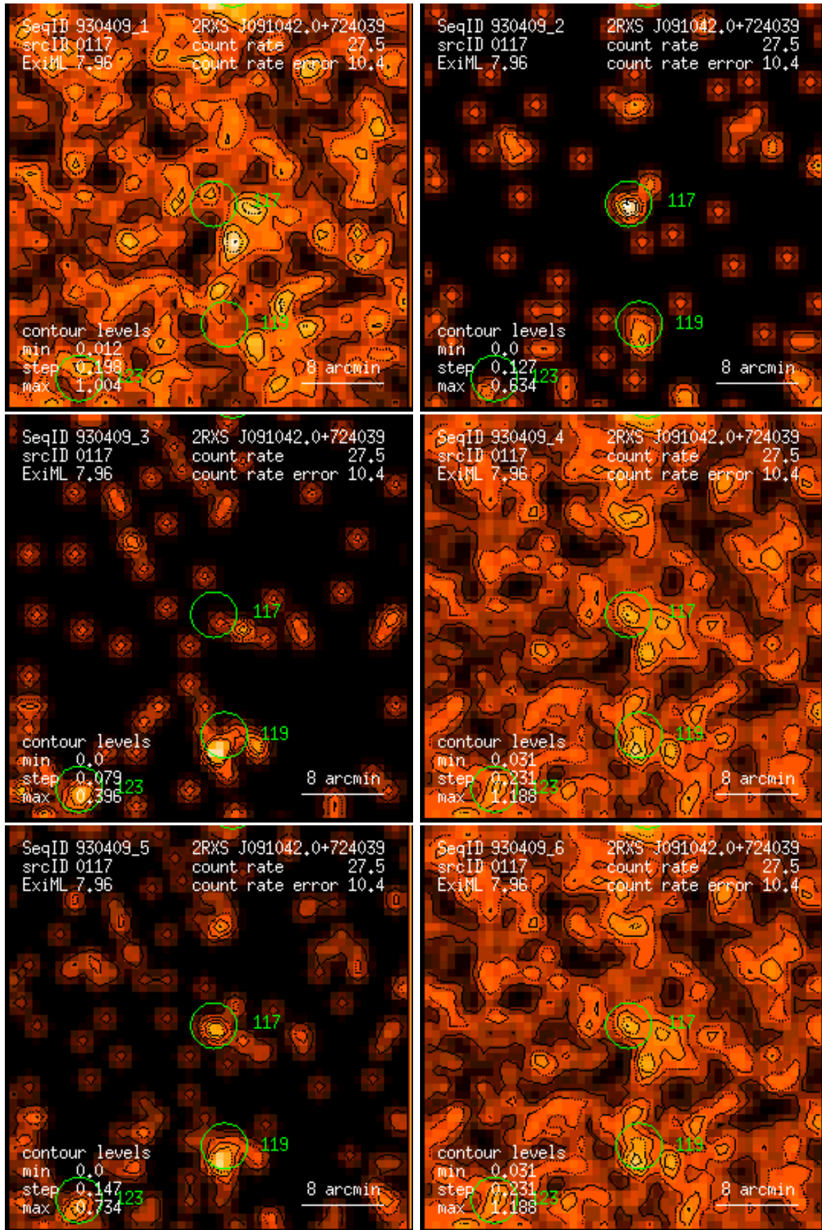
Figure 117: RASS 930409: detection 0117: band rate images, Gaussian filter: (1) PSPC channels 11 – 41, (2) 52 – 90, (3) 91 – 201, (4) 11 – 235, (5) 52 – 201, (6) 11 – 201. Broad band rates in counts/ks. Band rate contour levels in counts/ks/arcmin 2 .
