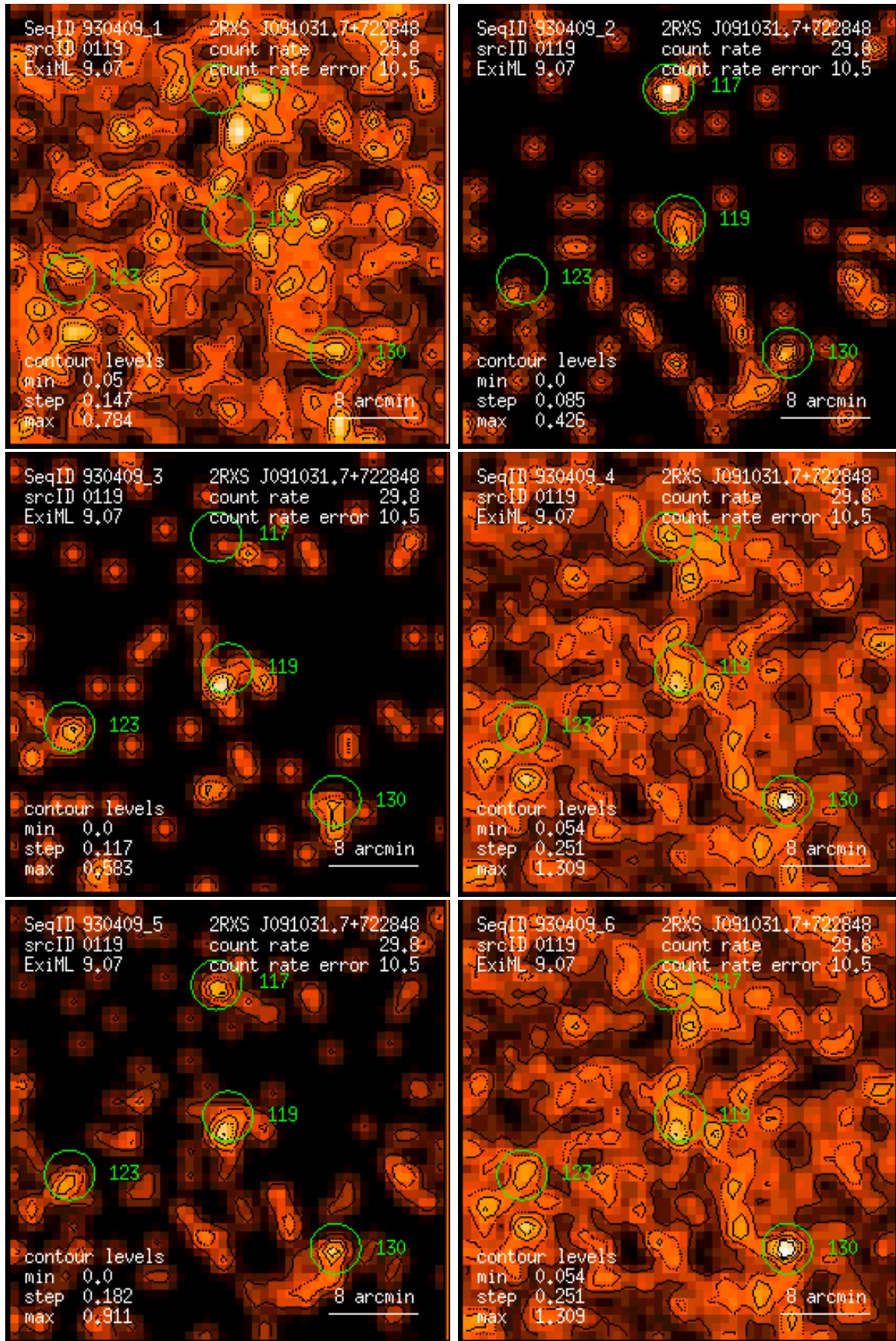
Figure 119: RASS 930409: detection 0119: band rate images, Gaussian filter: (1) PSPC channels 11 – 41, (2) 52 – 90, (3) 91 – 201, (4) 11 – 235, (5) 52 – 201, (6) 11 – 201. Broad band rates in counts/ks. Band rate contour levels in counts/ks/arcmin 2 .
