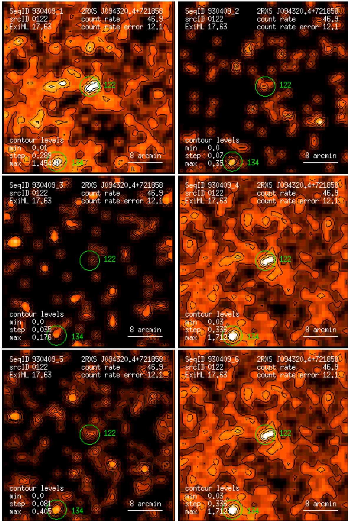
Figure 122: RASS 930409: detection 0122: band rate images, Gaussian filter: (1) PSPC channels 11 – 41, (2) 52 – 90, (3) 91 – 201, (4) 11 – 235, (5) 52 – 201, (6) 11 – 201. Broad band rates in counts/ks. Band rate contour levels in counts/ks/arcmin 2 .
