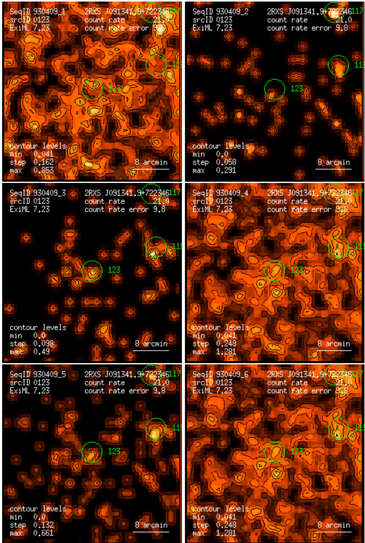
Figure 123: RASS 930409: detection 0123: band rate images, Gaussian filter: (1) PSPC channels 11 – 41, (2) 52 – 90, (3) 91 – 201, (4) 11 – 235, (5) 52 – 201, (6) 11 – 201. Broad band rates in counts/ks. Band rate contour levels in counts/ks/arcmin 2 .
