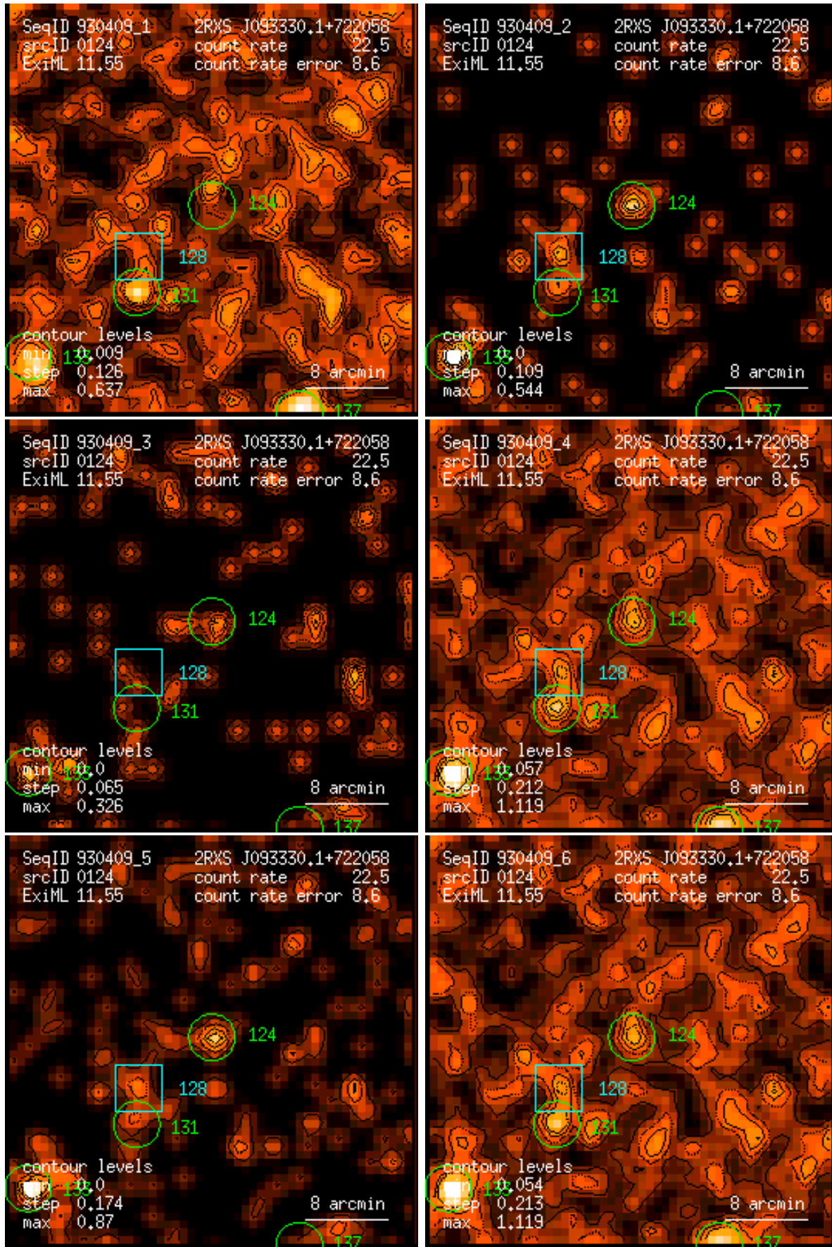
Figure 124: RASS 930409: detection 0124: band rate images, Gaussian filter: (1) PSPC channels 11 – 41, (2) 52 – 90, (3) 91 – 201, (4) 11 – 235, (5) 52 – 201, (6) 11 – 201. Broad band rates in counts/ks. Band rate contour levels in counts/ks/arcmin 2 .
