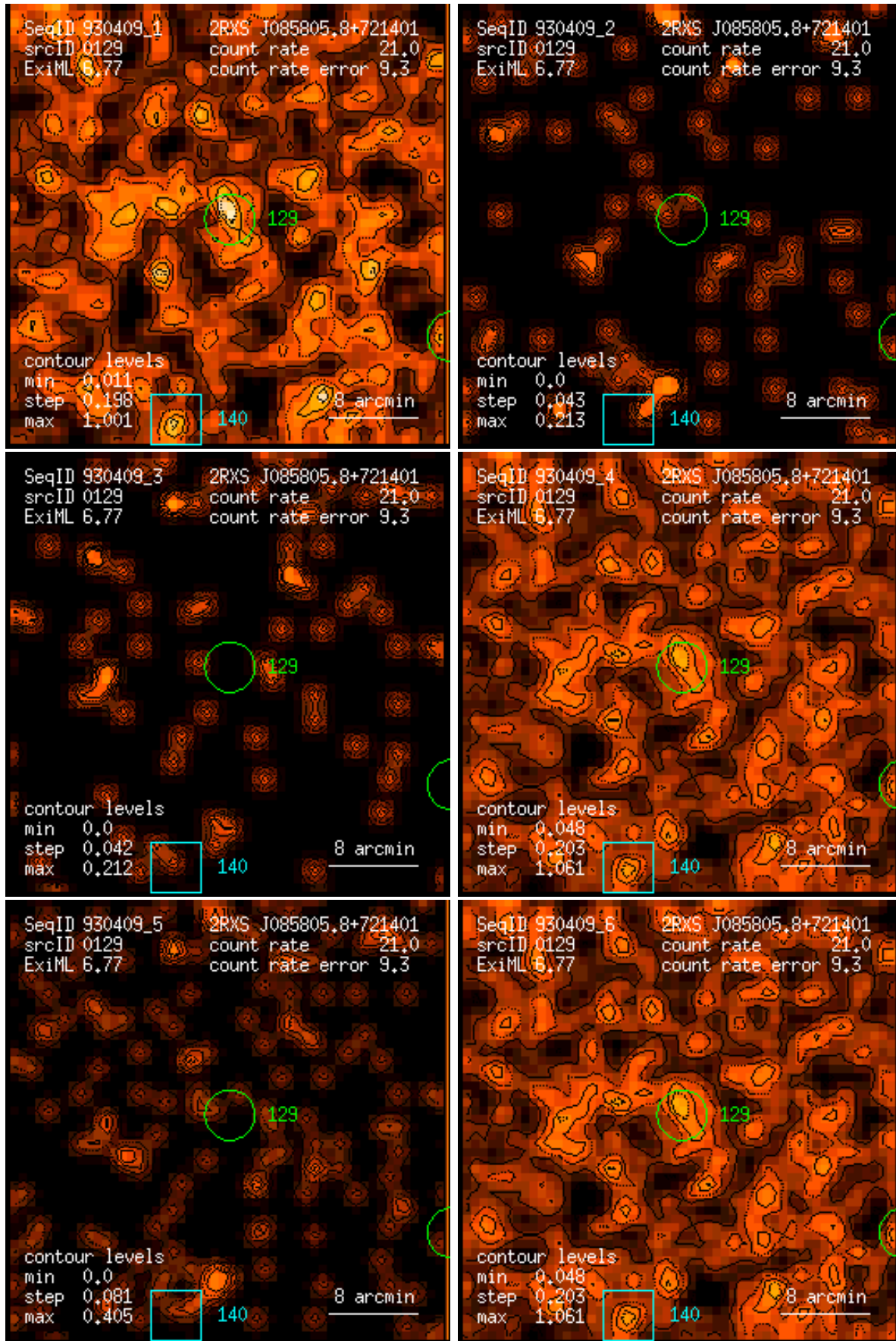
Figure 129: RASS 930409: detection 0129: band rate images, Gaussian filter: (1) PSPC channels 11 – 41, (2) 52 – 90, (3) 91 – 201, (4) 11 – 235, (5) 52 – 201, (6) 11 – 201. Broad band rates in counts/ks. Band rate contour levels in counts/ks/arcmin 2 .
