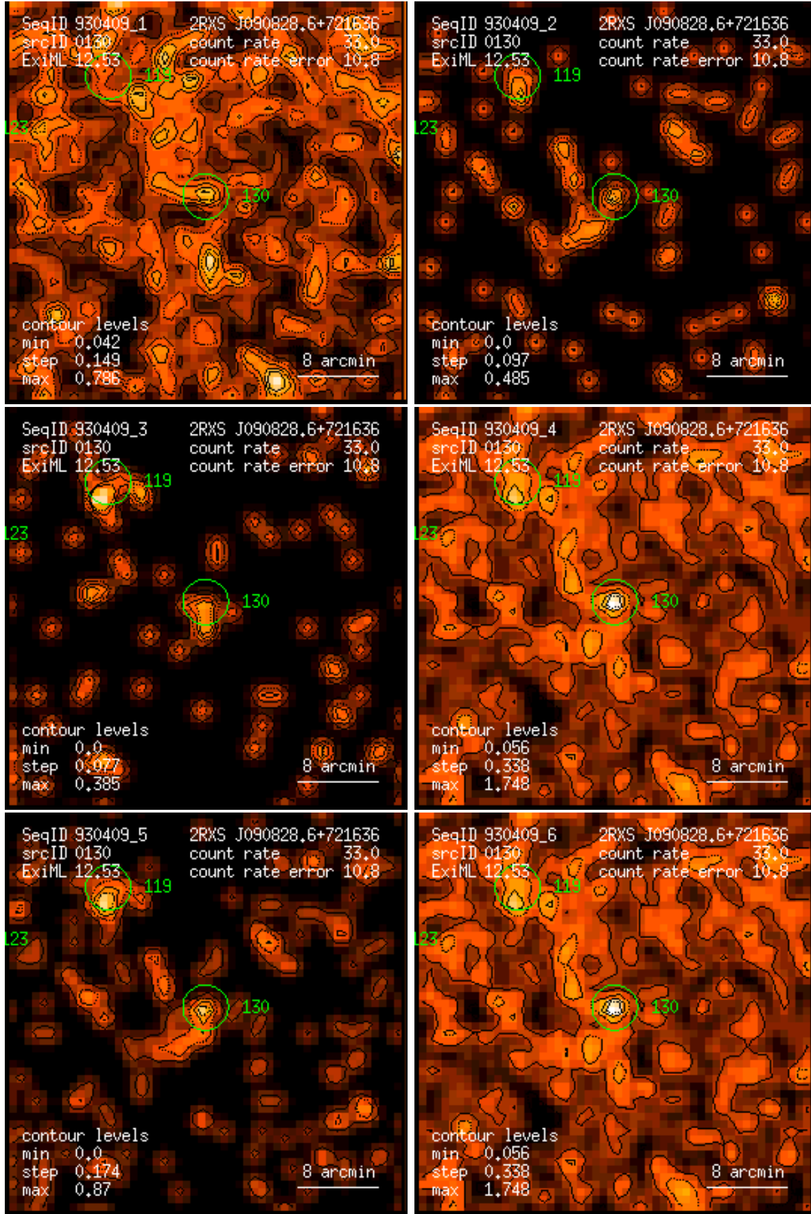
Figure 130: RASS 930409: detection 0130: band rate images, Gaussian filter: (1) PSPC channels 11 – 41, (2) 52 – 90, (3) 91 – 201, (4) 11 – 235, (5) 52 – 201, (6) 11 – 201. Broad band rates in counts/ks. Band rate contour levels in counts/ks/arcmin 2 .
