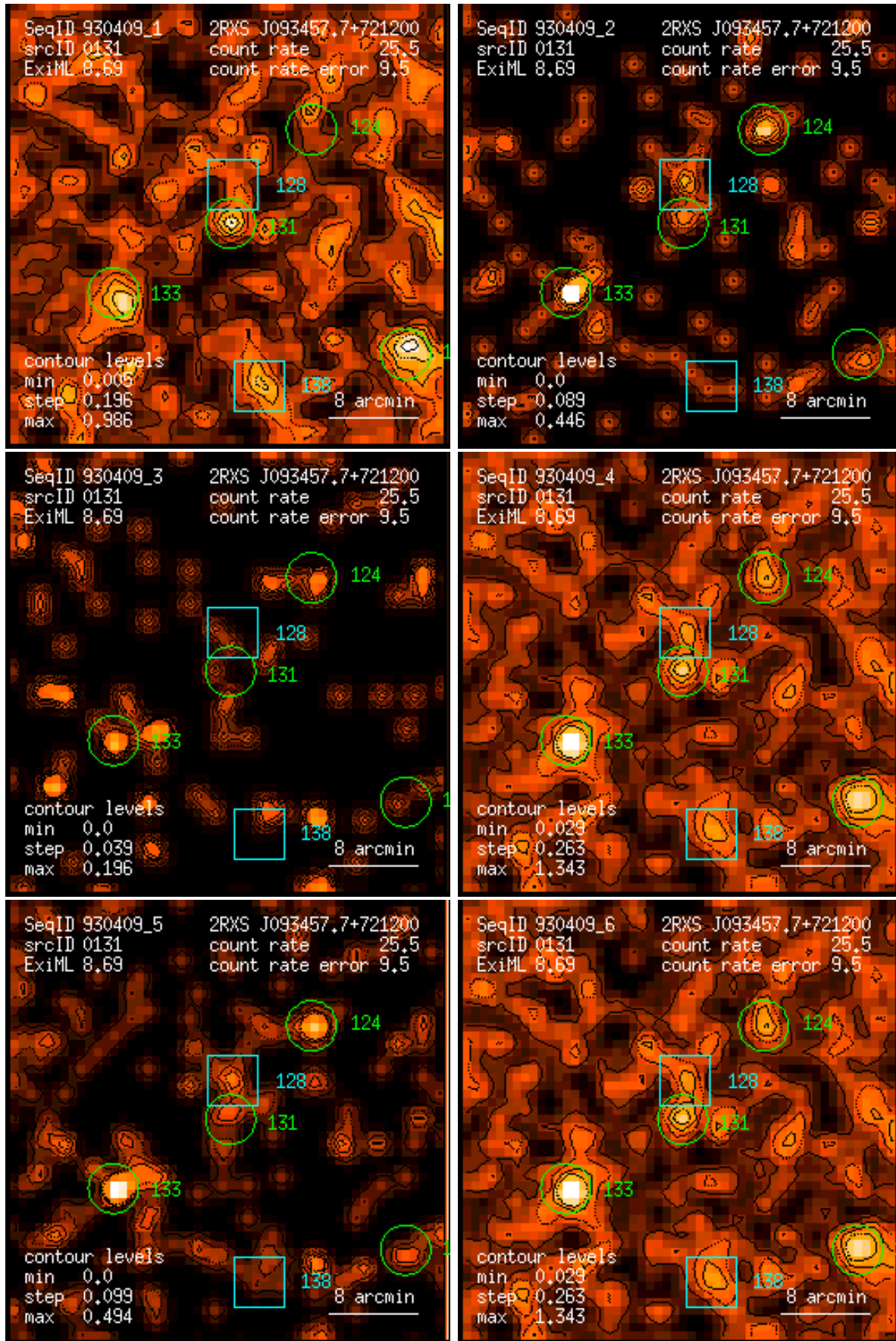
Figure 131: RASS 930409: detection 0131: band rate images, Gaussian filter: (1) PSPC channels 11 – 41, (2) 52 – 90, (3) 91 – 201, (4) 11 – 235, (5) 52 – 201, (6) 11 – 201. Broad band rates in counts/ks. Band rate contour levels in counts/ks/arcmin 2 .
