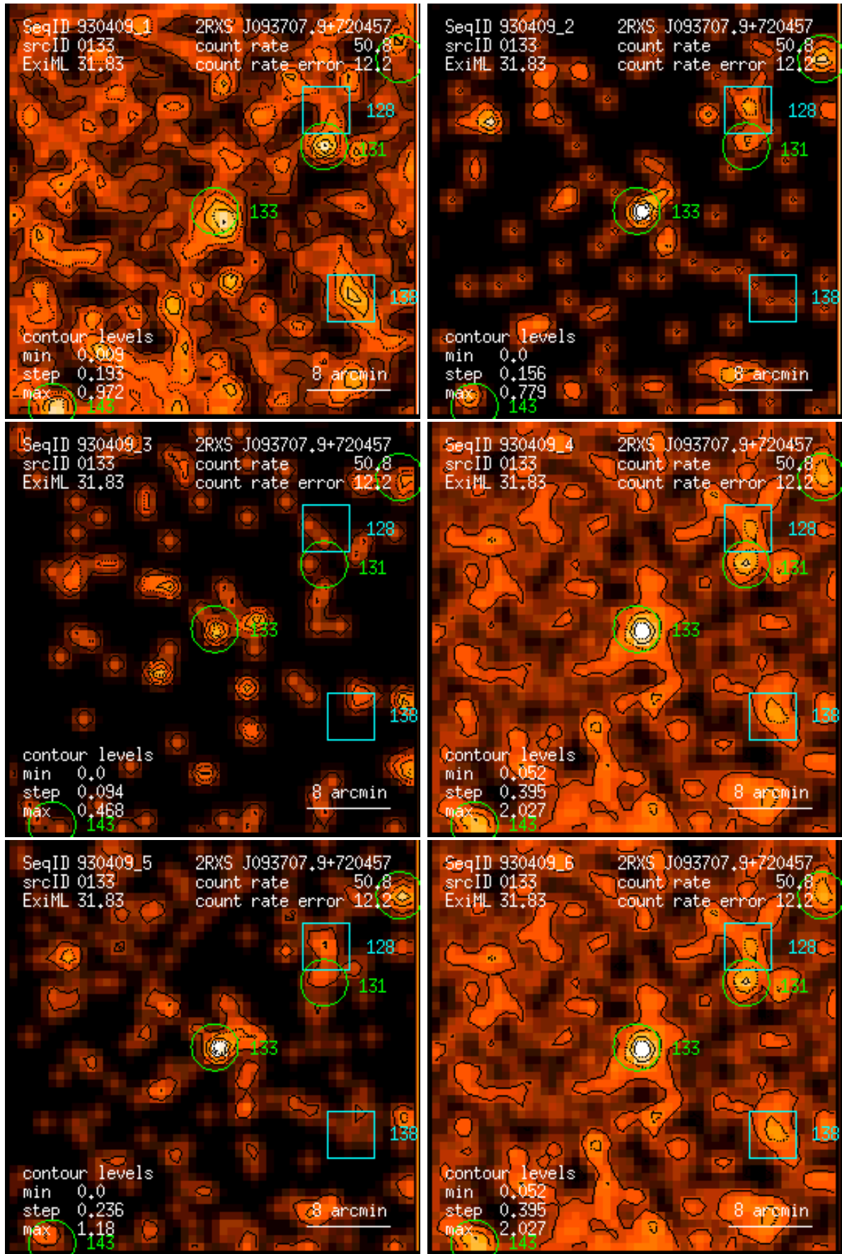
Figure 133: RASS 930409: detection 0133: band rate images, Gaussian filter: (1) PSPC channels 11 – 41, (2) 52 – 90, (3) 91 – 201, (4) 11 – 235, (5) 52 – 201, (6) 11 – 201. Broad band rates in counts/ks. Band rate contour levels in counts/ks/arcmin 2 .
