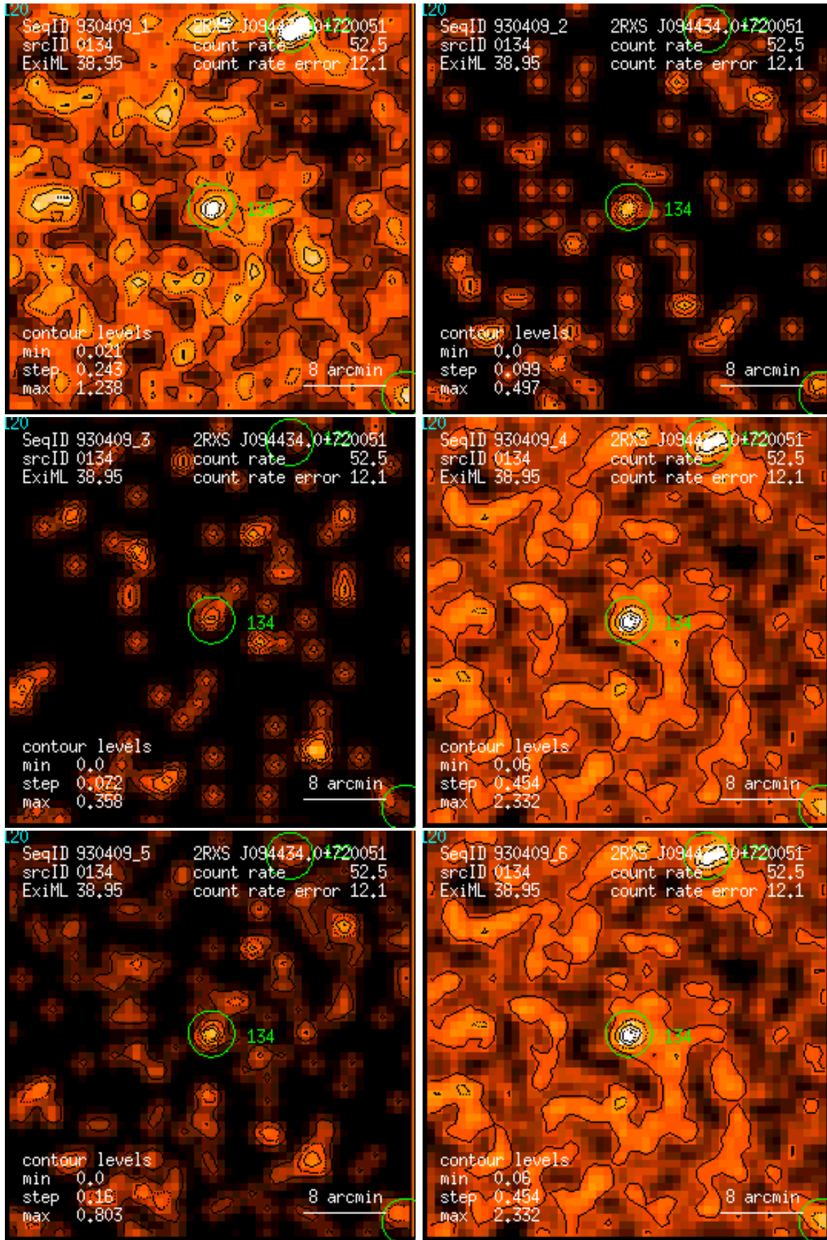
Figure 134: RASS 930409: detection 0134: band rate images, Gaussian filter: (1) PSPC channels 11 – 41, (2) 52 – 90, (3) 91 – 201, (4) 11 – 235, (5) 52 – 201, (6) 11 – 201. Broad band rates in counts/ks. Band rate contour levels in counts/ks/arcmin 2 .
