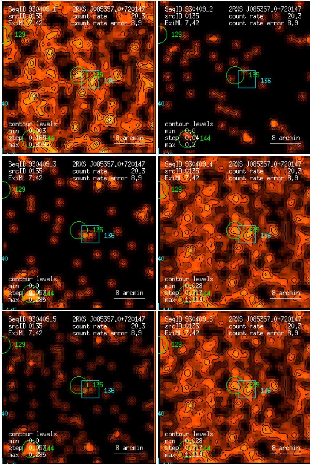
Figure 135: RASS 930409: detection 0135: band rate images, Gaussian filter: (1) PSPC channels 11 – 41, (2) 52 – 90, (3) 91 – 201, (4) 11 – 235, (5) 52 – 201, (6) 11 – 201. Broad band rates in counts/ks. Band rate contour levels in counts/ks/arcmin 2 .
