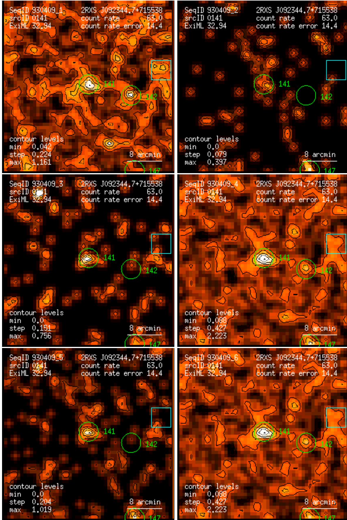
Figure 141: RASS 930409: detection 0141: band rate images, Gaussian filter: (1) PSPC channels 11 – 41, (2) 52 – 90, (3) 91 – 201, (4) 11 – 235, (5) 52 – 201, (6) 11 – 201. Broad band rates in counts/ks. Band rate contour levels in counts/ks/arcmin 2 .
