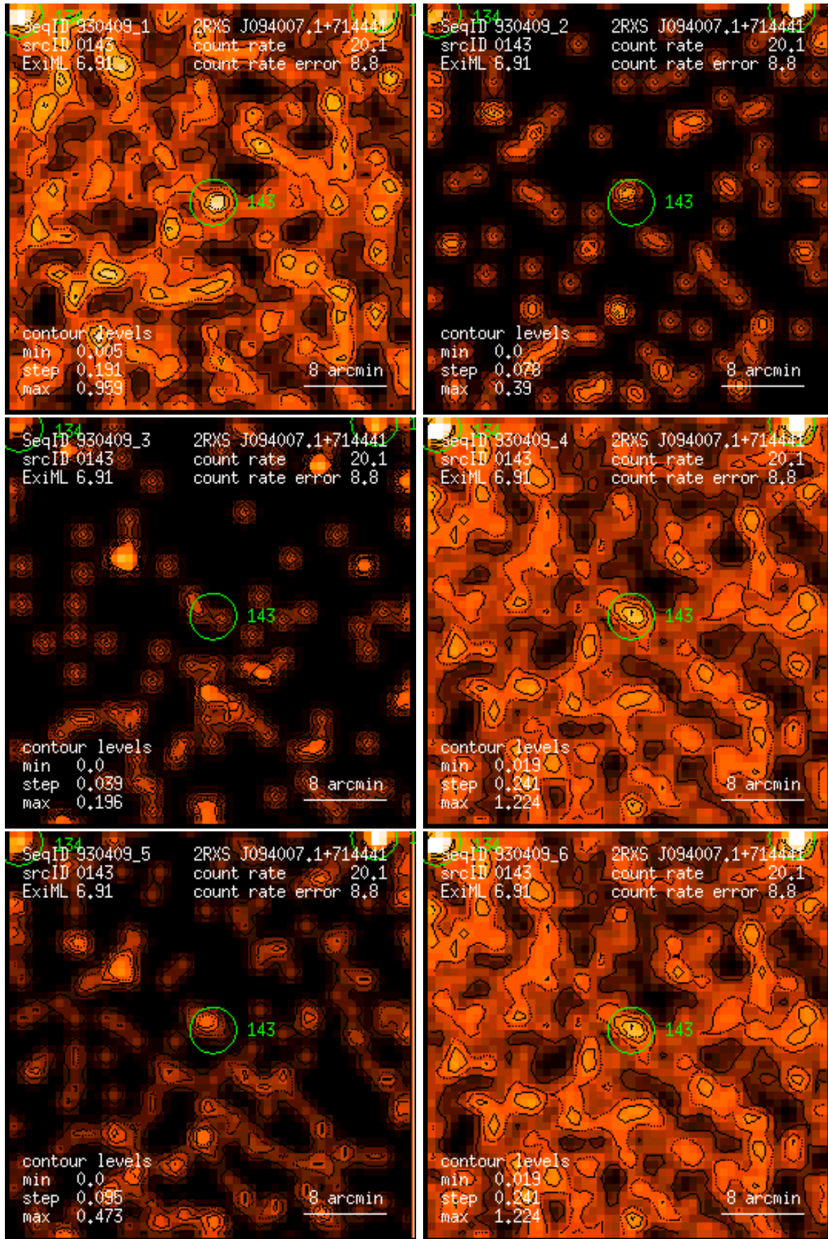
Figure 143: RASS 930409: detection 0143: band rate images, Gaussian filter: (1) PSPC channels 11 – 41, (2) 52 – 90, (3) 91 – 201, (4) 11 – 235, (5) 52 – 201, (6) 11 – 201. Broad band rates in counts/ks. Band rate contour levels in counts/ks/arcmin 2 .
