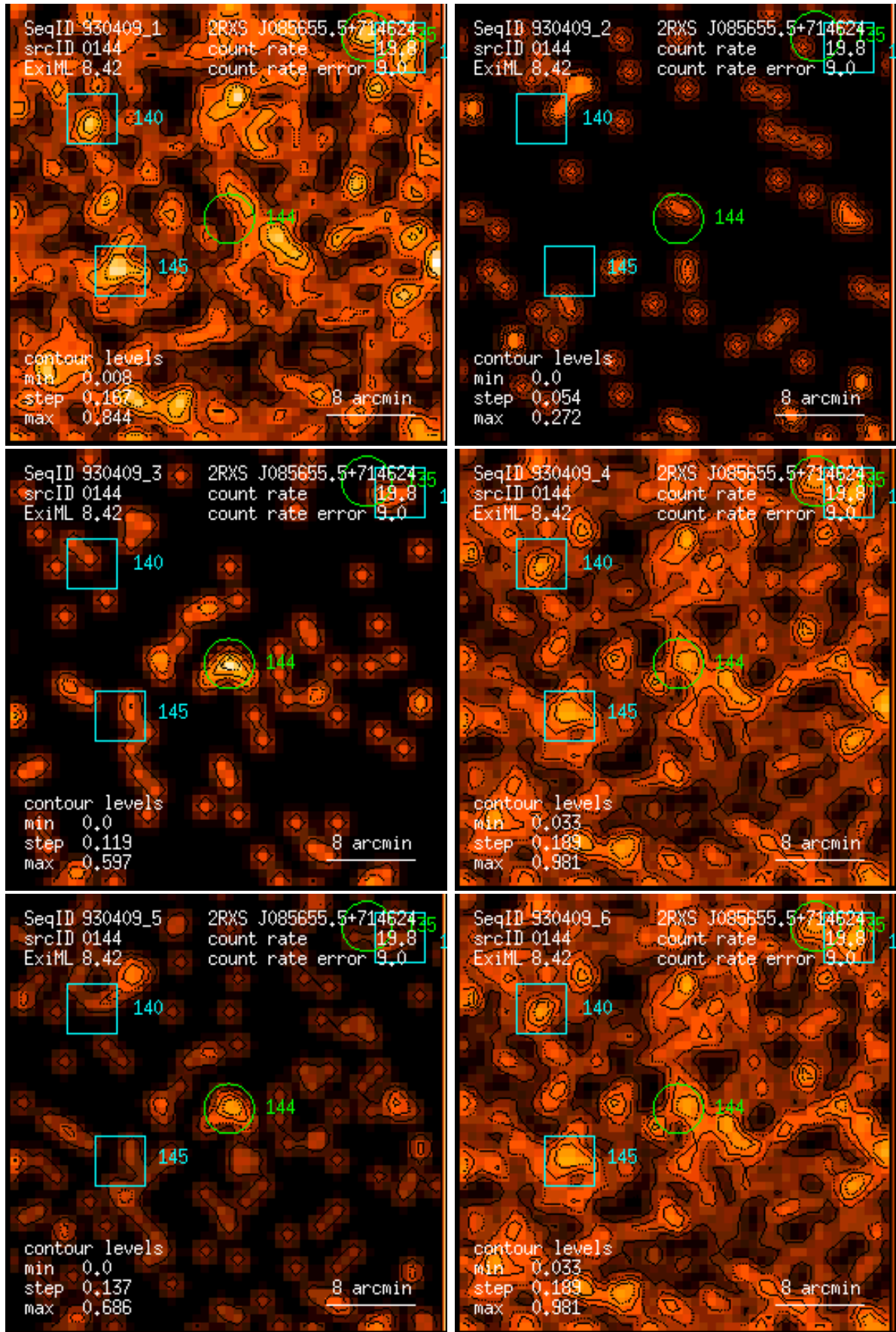
Figure 144: RASS 930409: detection 0144: band rate images, Gaussian filter: (1) PSPC channels 11 – 41, (2) 52 – 90, (3) 91 – 201, (4) 11 – 235, (5) 52 – 201, (6) 11 – 201. Broad band rates in counts/ks. Band rate contour levels in counts/ks/arcmin 2 .
