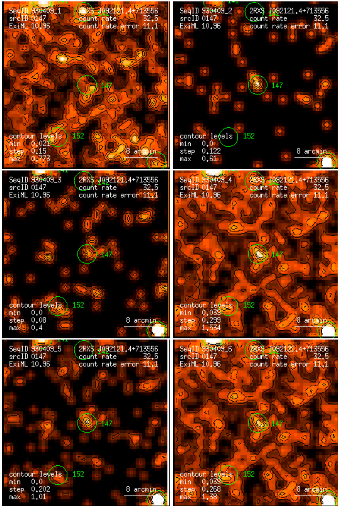
Figure 147: RASS 930409: detection 0147: band rate images, Gaussian filter: (1) PSPC channels 11 – 41, (2) 52 – 90, (3) 91 – 201, (4) 11 – 235, (5) 52 – 201, (6) 11 – 201. Broad band rates in counts/ks. Band rate contour levels in counts/ks/arcmin 2 .
