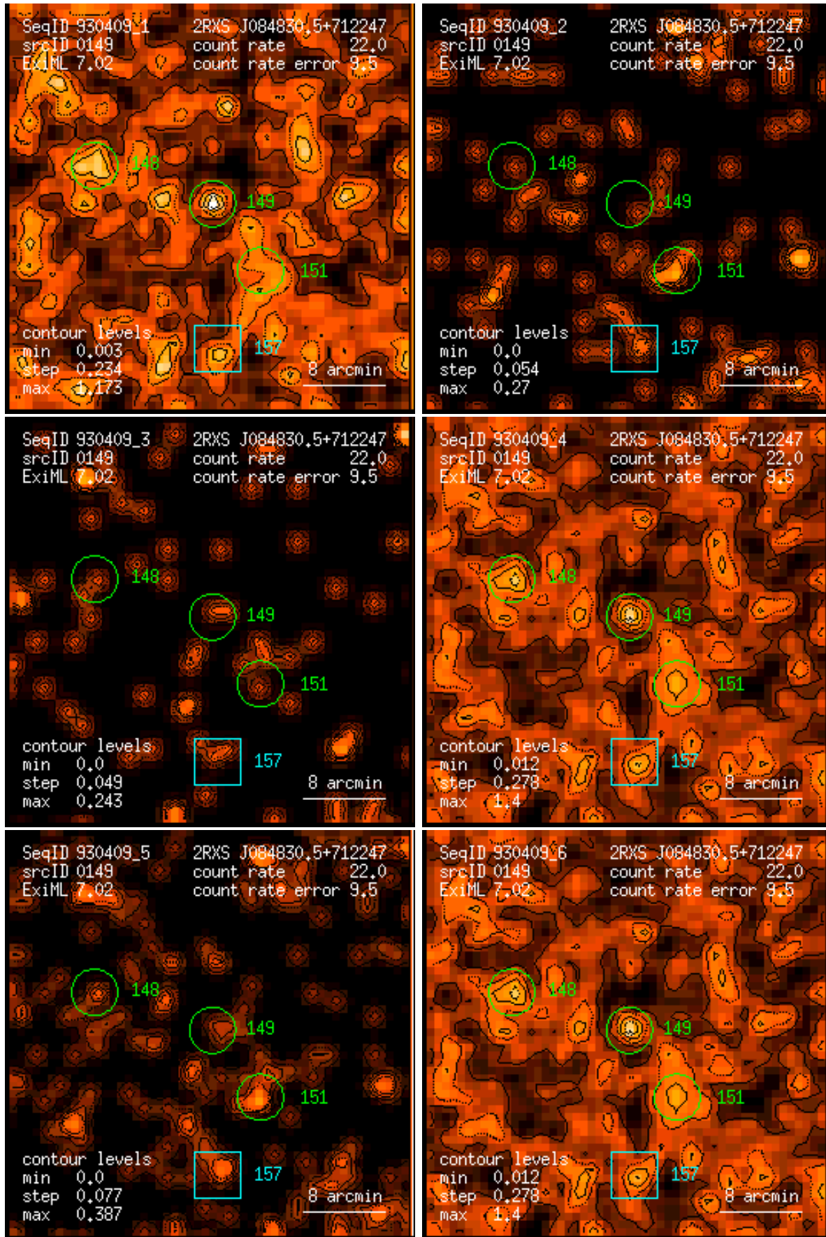
Figure 149: RASS 930409: detection 0149: band rate images, Gaussian filter: (1) PSPC channels 11 – 41, (2) 52 – 90, (3) 91 – 201, (4) 11 – 235, (5) 52 – 201, (6) 11 – 201. Broad band rates in counts/ks. Band rate contour levels in counts/ks/arcmin 2 .
