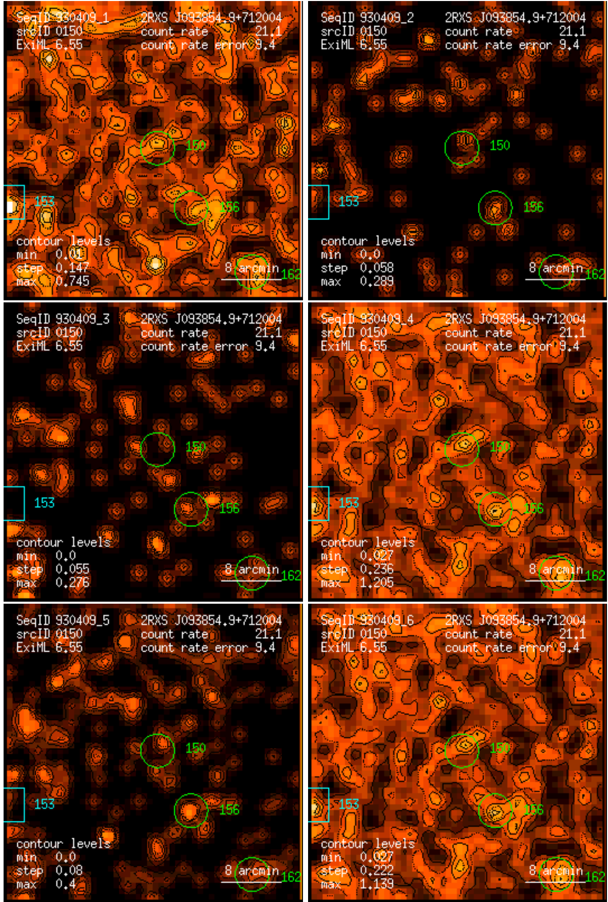
Figure 150: RASS 930409: detection 0150: band rate images, Gaussian filter: (1) PSPC channels 11 – 41, (2) 52 – 90, (3) 91 – 201, (4) 11 – 235, (5) 52 – 201, (6) 11 – 201. Broad band rates in counts/ks. Band rate contour levels in counts/ks/arcmin 2 .
