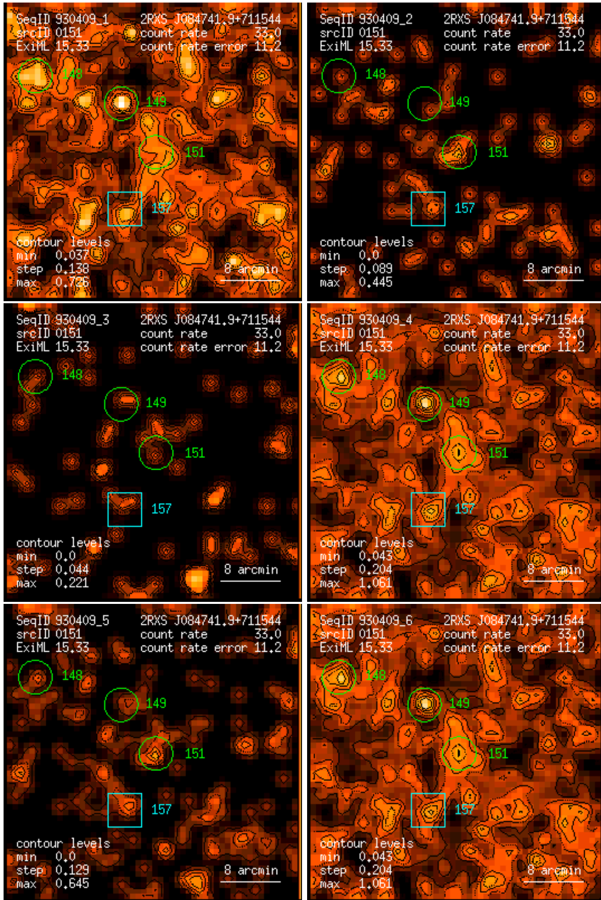
Figure 151: RASS 930409: detection 0151: band rate images, Gaussian filter: (1) PSPC channels 11 – 41, (2) 52 – 90, (3) 91 – 201, (4) 11 – 235, (5) 52 – 201, (6) 11 – 201. Broad band rates in counts/ks. Band rate contour levels in counts/ks/arcmin 2 .
