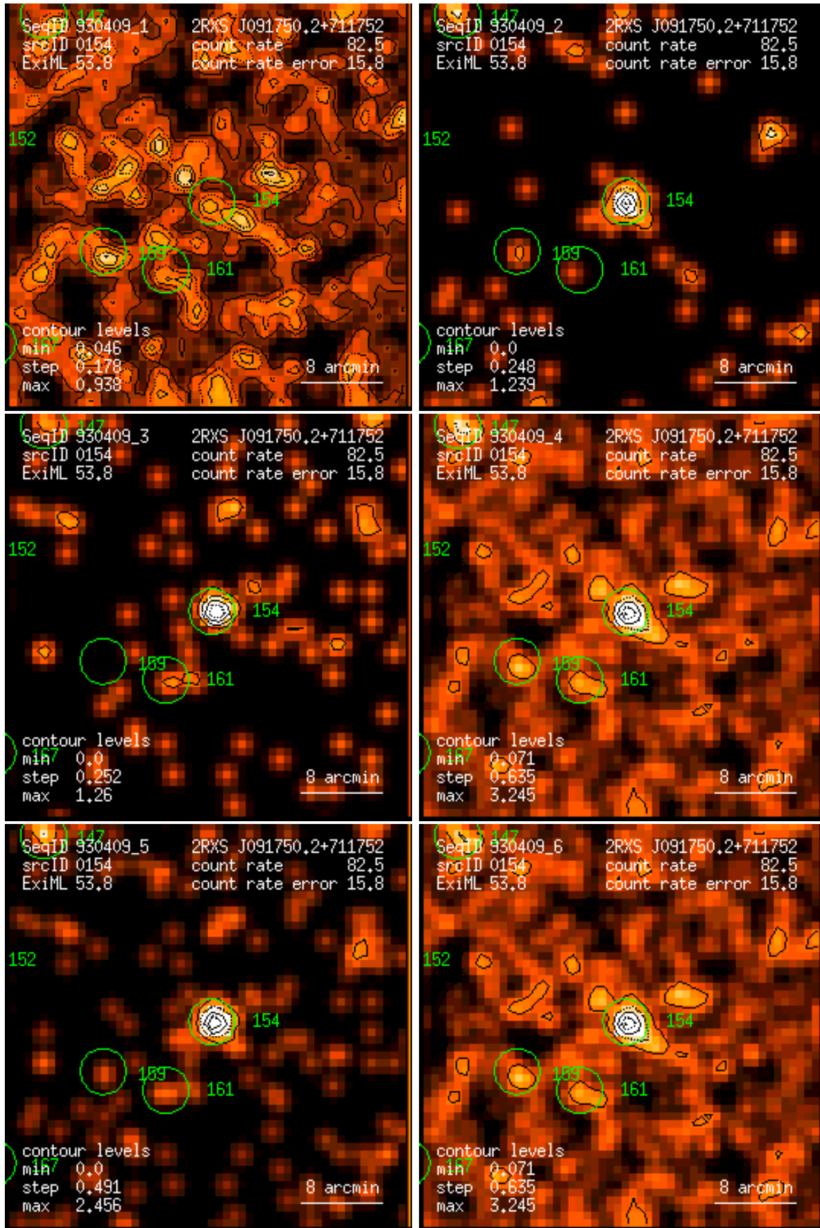
Figure 154: RASS 930409: detection 0154: band rate images, Gaussian filter: (1) PSPC channels 11 – 41, (2) 52 – 90, (3) 91 – 201, (4) 11 – 235, (5) 52 – 201, (6) 11 – 201. Broad band rates in counts/ks. Band rate contour levels in counts/ks/arcmin 2 .
