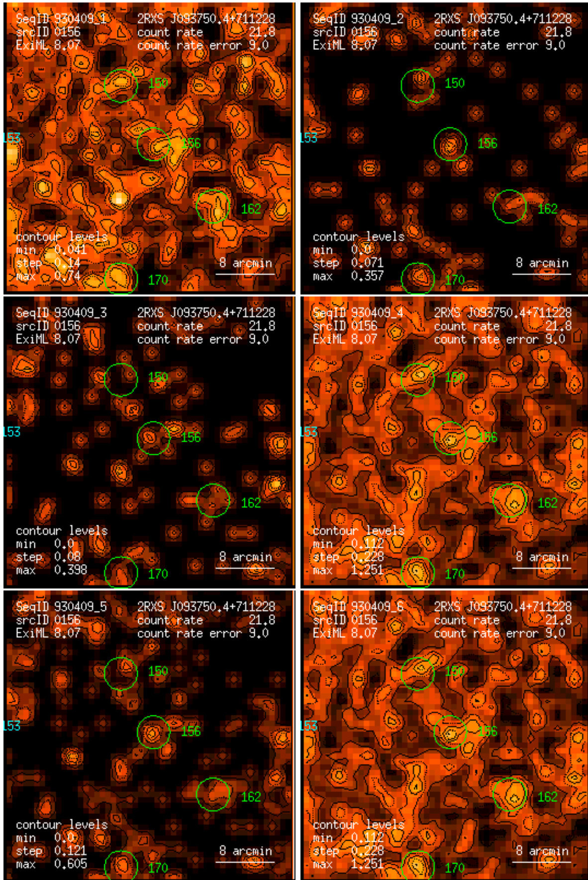
Figure 156: RASS 930409: detection 0156: band rate images, Gaussian filter: (1) PSPC channels 11 – 41, (2) 52 – 90, (3) 91 – 201, (4) 11 – 235, (5) 52 – 201, (6) 11 – 201. Broad band rates in counts/ks. Band rate contour levels in counts/ks/arcmin 2 .
