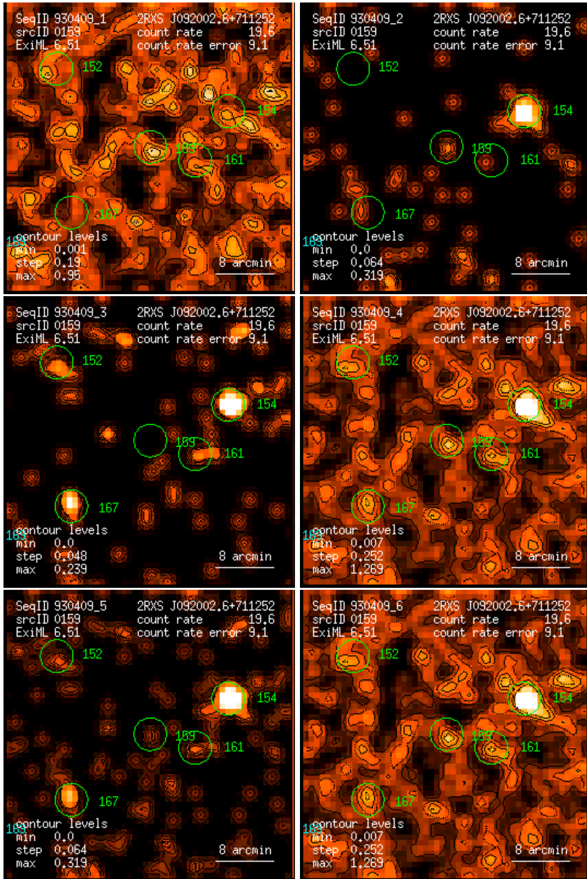
Figure 159: RASS 930409: detection 0159: band rate images, Gaussian filter: (1) PSPC channels 11 – 41, (2) 52 – 90, (3) 91 – 201, (4) 11 – 235, (5) 52 – 201, (6) 11 – 201. Broad band rates in counts/ks. Band rate contour levels in counts/ks/arcmin 2 .
