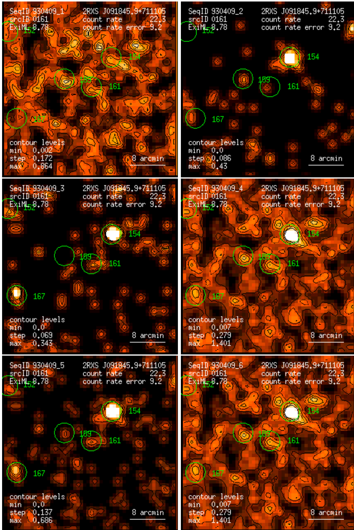
Figure 161: RASS 930409: detection 0161: band rate images, Gaussian filter: (1) PSPC channels 11 – 41, (2) 52 – 90, (3) 91 – 201, (4) 11 – 235, (5) 52 – 201, (6) 11 – 201. Broad band rates in counts/ks. Band rate contour levels in counts/ks/arcmin 2 .
