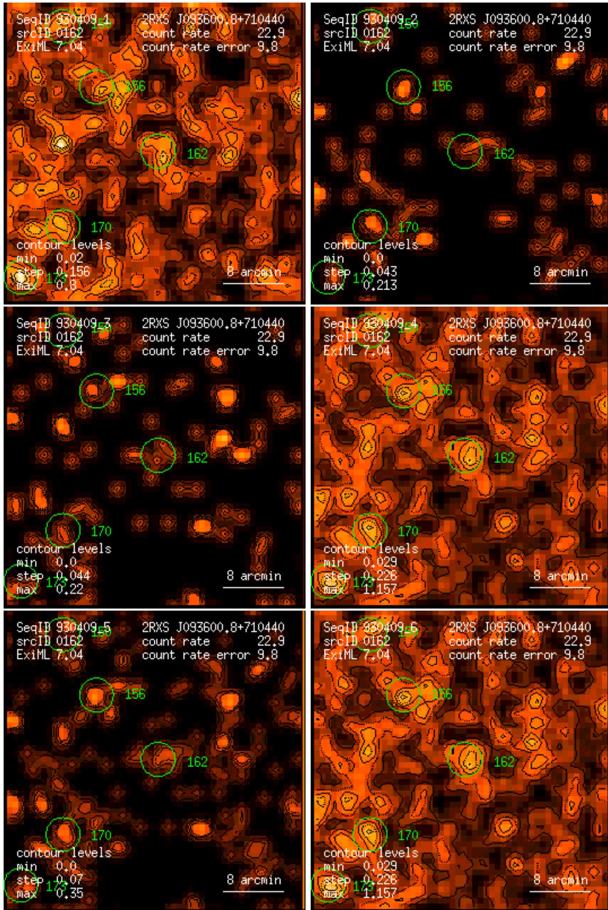
Figure 162: RASS 930409: detection 0162: band rate images, Gaussian filter: (1) PSPC channels 11 – 41, (2) 52 – 90, (3) 91 – 201, (4) 11 – 235, (5) 52 – 201, (6) 11 – 201. Broad band rates in counts/ks. Band rate contour levels in counts/ks/arcmin 2 .
