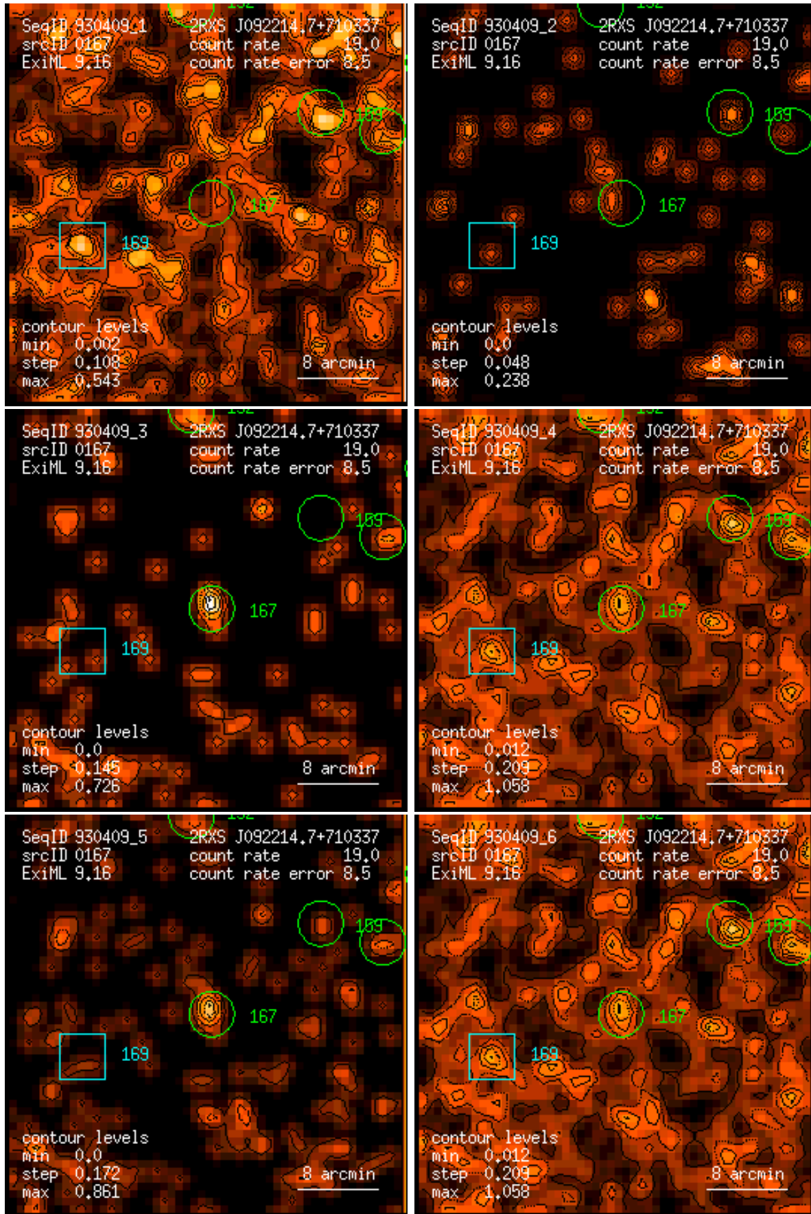
Figure 167: RASS 930409: detection 0167: band rate images, Gaussian filter: (1) PSPC channels 11 – 41, (2) 52 – 90, (3) 91 – 201, (4) 11 – 235, (5) 52 – 201, (6) 11 – 201. Broad band rates in counts/ks. Band rate contour levels in counts/ks/arcmin 2 .
