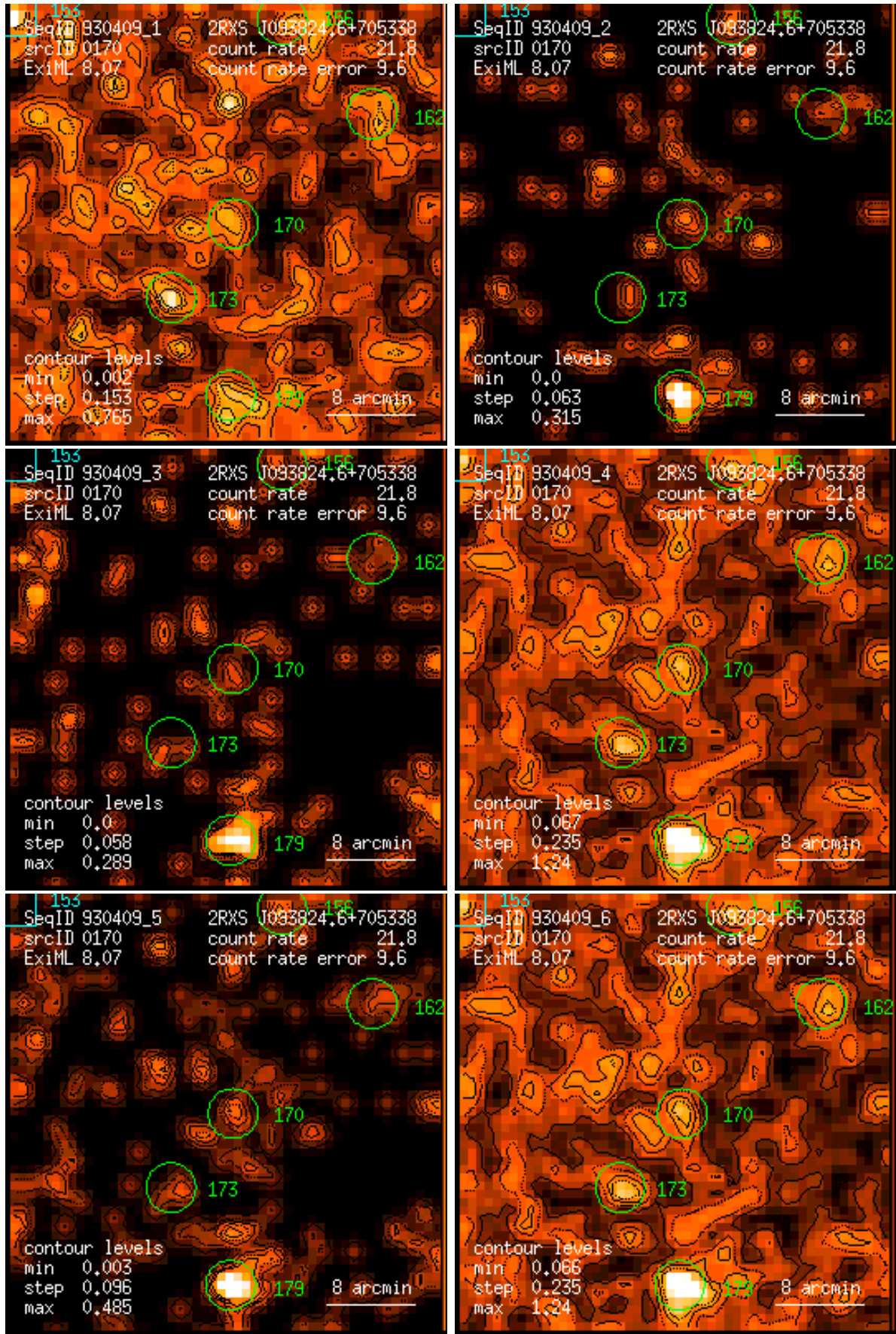
Figure 170: RASS 930409: detection 0170: band rate images, Gaussian filter: (1) PSPC channels 11 – 41, (2) 52 – 90, (3) 91 – 201, (4) 11 – 235, (5) 52 – 201, (6) 11 – 201. Broad band rates in counts/ks. Band rate contour levels in counts/ks/arcmin 2 .
