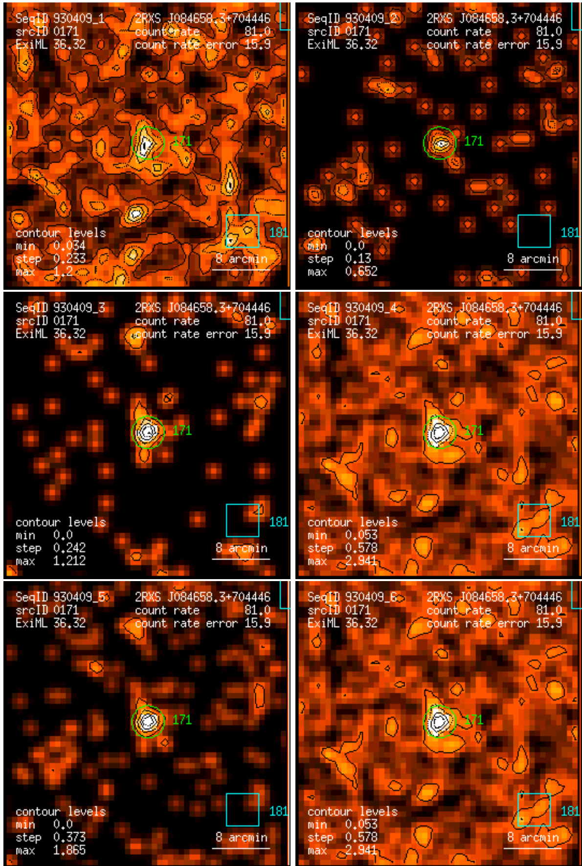
Figure 171: RASS 930409: detection 0171: band rate images, Gaussian filter: (1) PSPC channels 11 – 41, (2) 52 – 90, (3) 91 – 201, (4) 11 – 235, (5) 52 – 201, (6) 11 – 201. Broad band rates in counts/ks. Band rate contour levels in counts/ks/arcmin 2 .
